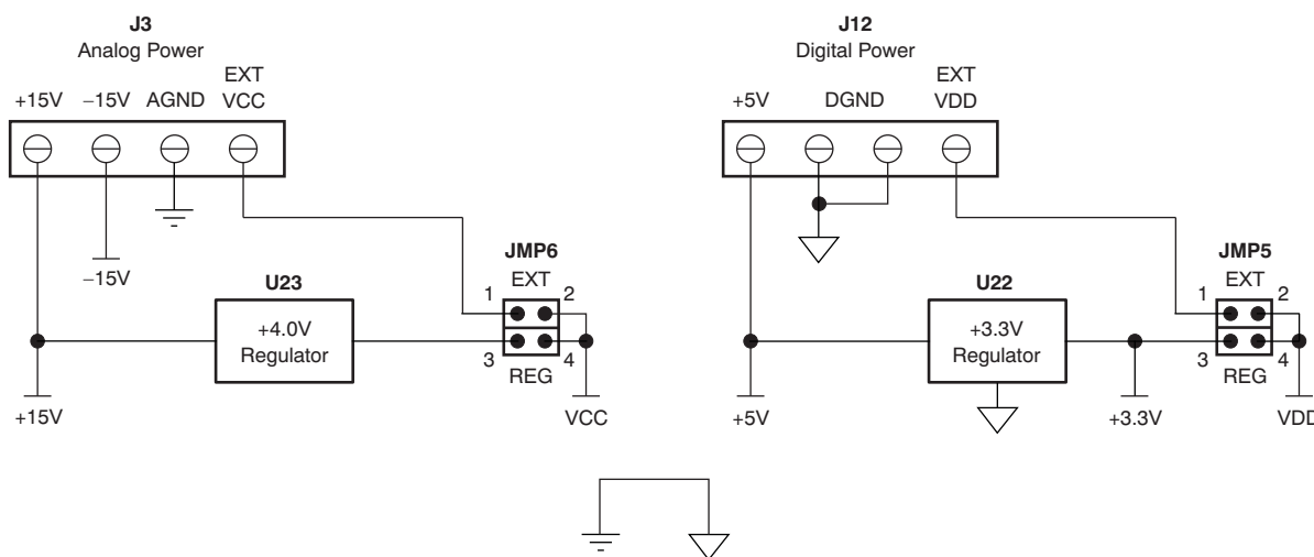
Figure 3. Power Supply Jumper Configuration
