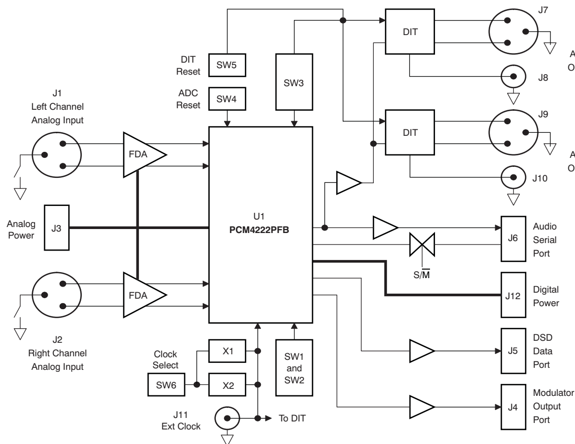
Figure 2. Simplified Block Diagram for the PCM4222EVM Evaluation Module
