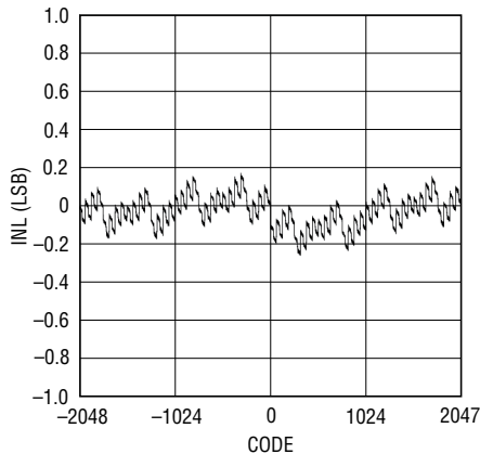
LTC1854 Typical INL Curve
