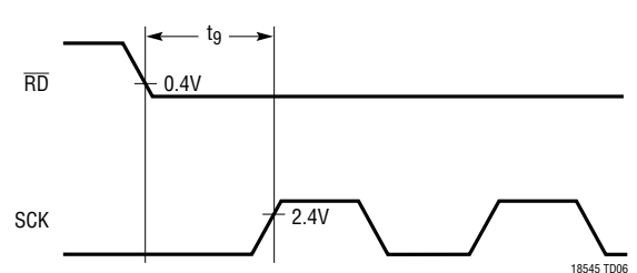
t 9 ( \overline{\text{RD}} ↓ to SCK Setup Time)
