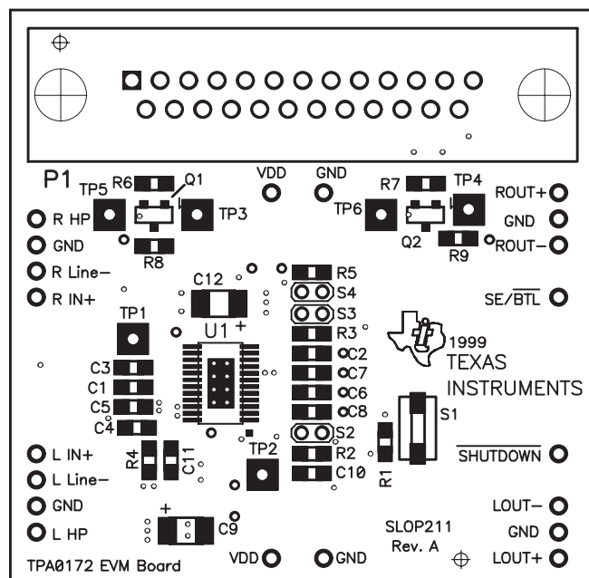
Figure 2–7. TPA0172 EVM Silkscreen
