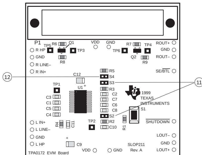
Figure 2–2. Module Map
