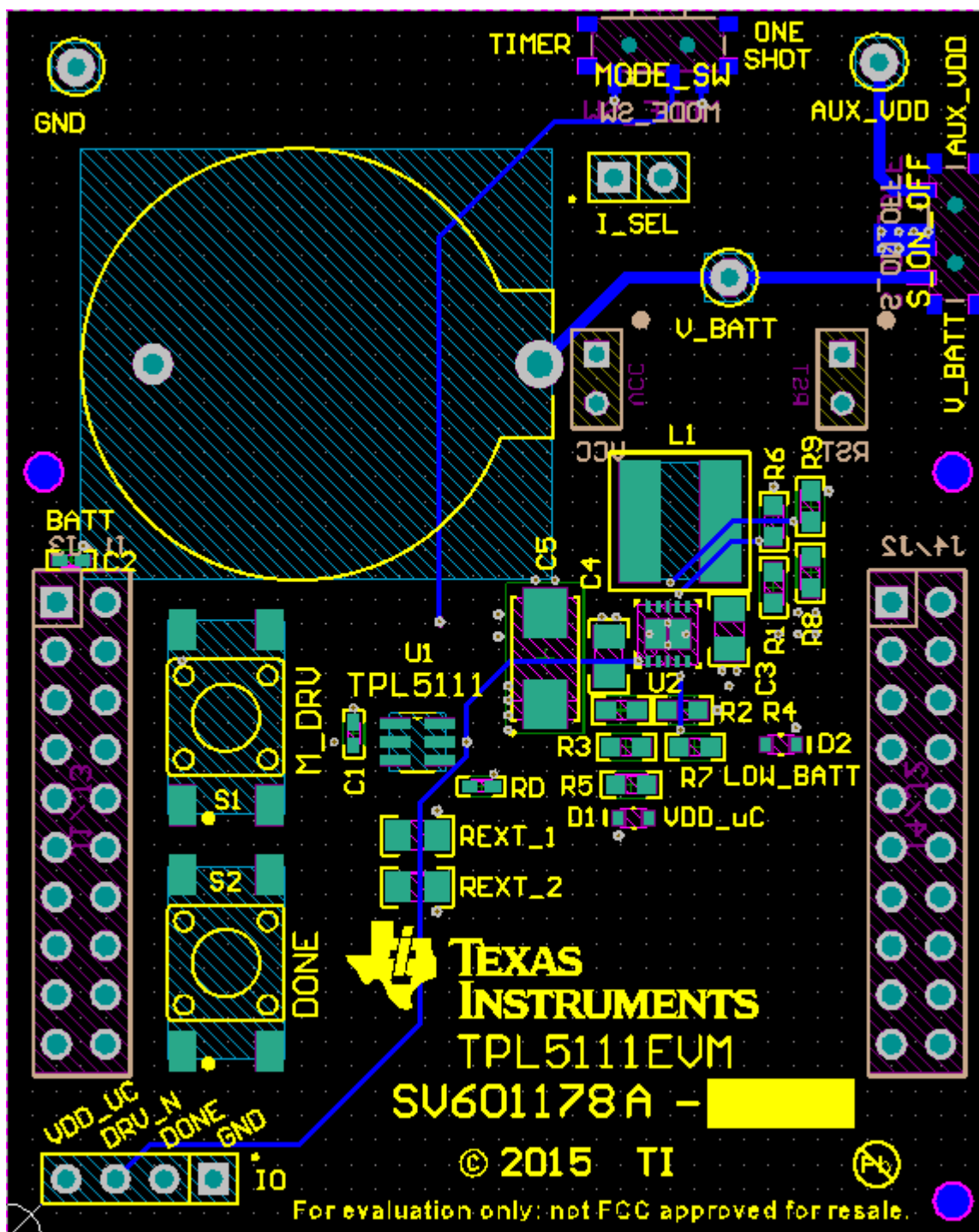
Figure 10. Bottom Layer
