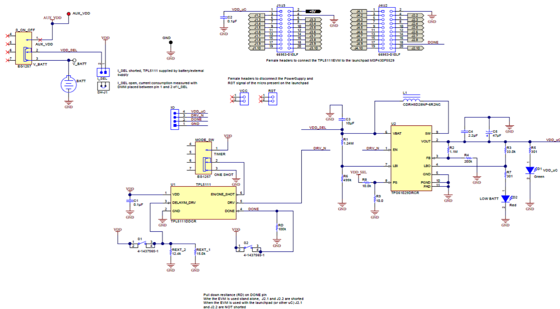
Figure 11. TPL5111EVM Schematic
