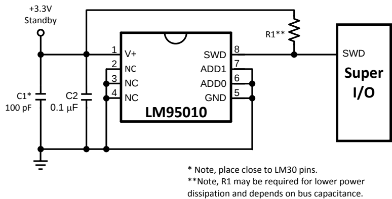
Figure 2. LM95010 connection to SensorPath master such as a Super I/O.
