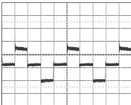
Figure 30. Output Ripple
