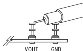
Figure 3. Correct Method For Measuring Input or Output Voltage Ripple
