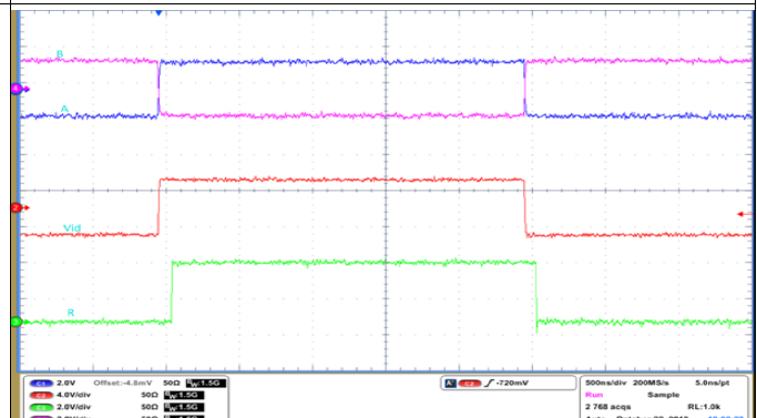
Figure 30. ISO143x Driver Propagation Delay
