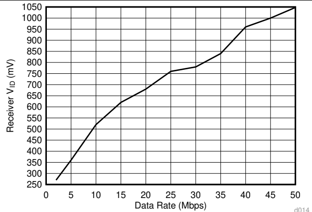
Figure 28. ISO145x Receiver V_{ID} vs Signaling Rate
