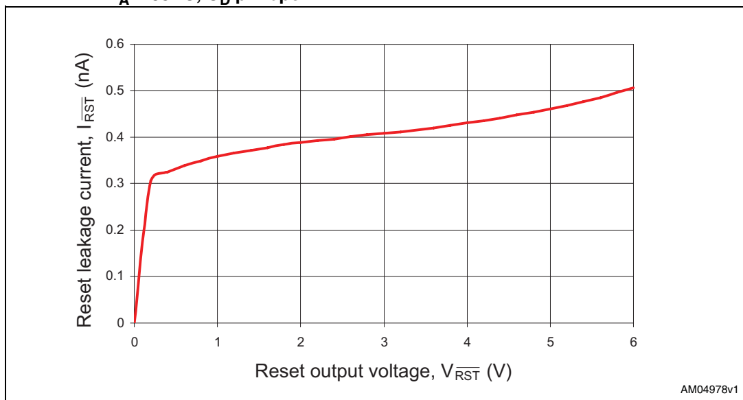
Figure 19. \overline{\text{RST}} output leakage current vs. output voltage, V_{\text{CC}} = V_{\text{SEN}} = 6.0 \text{ V} , T_A = 85^\circ\text{C} , C_{\text{D}} pin open
