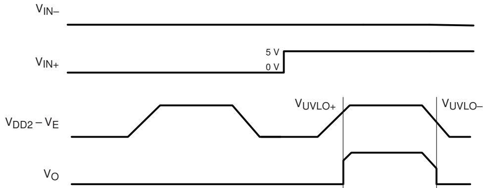
Figure 59. UVLO for Output Side
