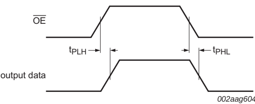
Fig 17. Output propagation delay
