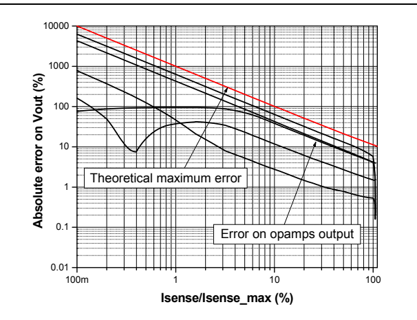
Figure 7. Absolute error on the output voltage vs. I_{sense}/I_{max} using an alternative op amp
