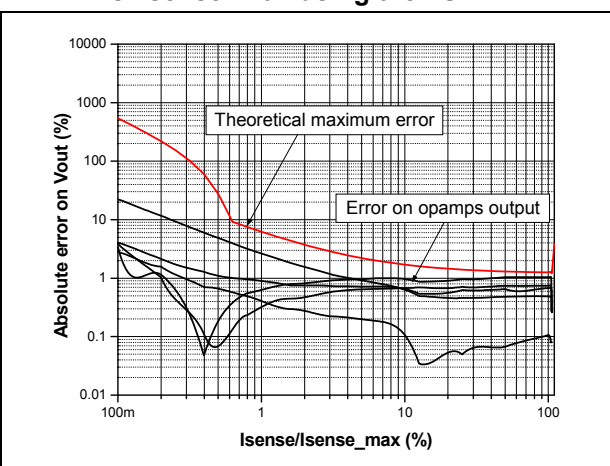
Figure 5. Absolute error on the output voltage vs. I_{sense}/I_{max} using the TSZ121
