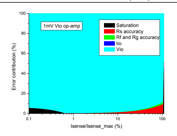
Figure 9. Contribution of each parameter to overall error for a 1 mV V_{io} op amp
