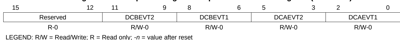
Figure 7-116. Trip-Zone Digital Compare Event Select Register (TZDCSEL)
