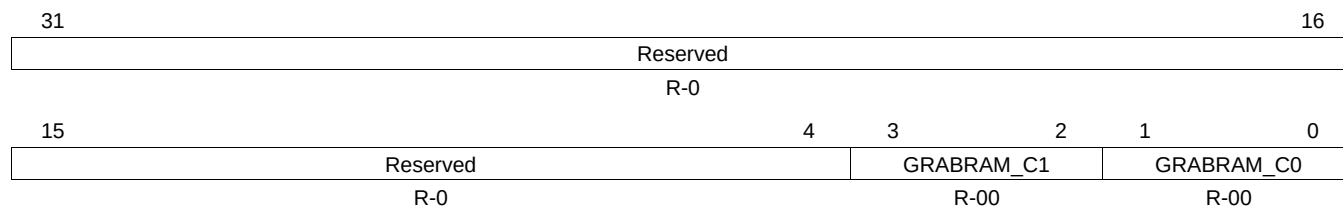
Figure 1-147. Z1_GRABRAMR Register
