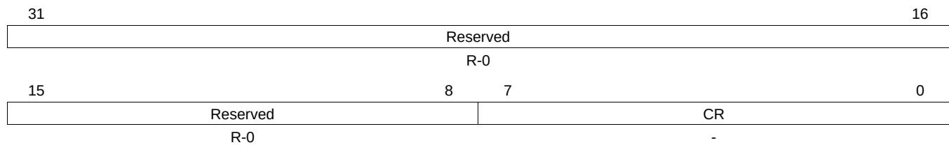
Figure 4-18. GPIO Commit (GPIOCR) Register
