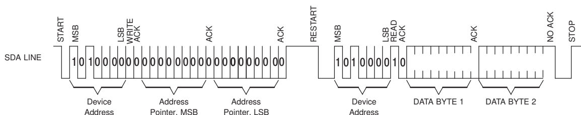
Figure 6-26. Sequential Read
