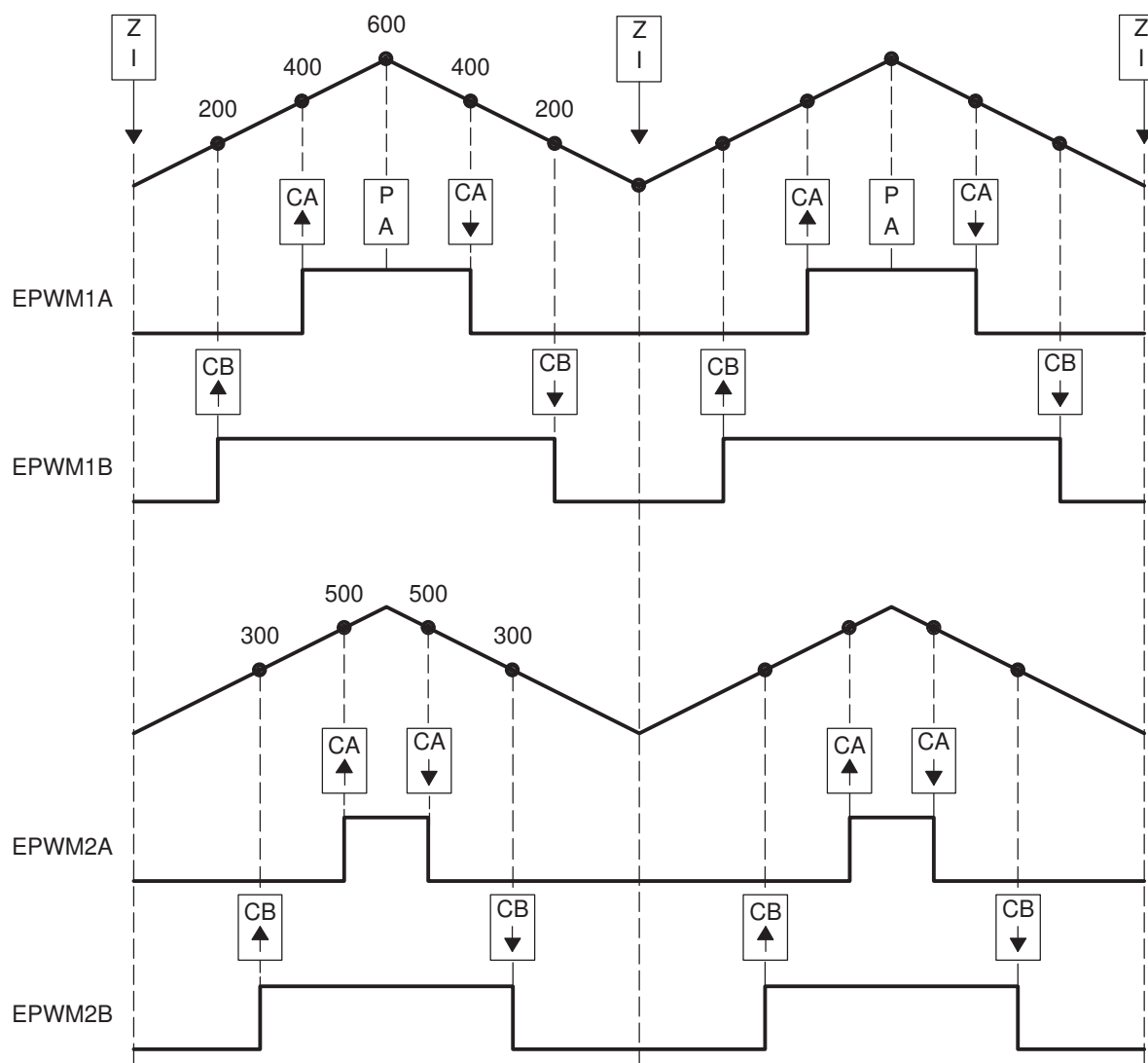
Figure 7-60. Buck Waveforms for Figure 7-59 (Note: F_{PWM2} = F_{PWM1} )
