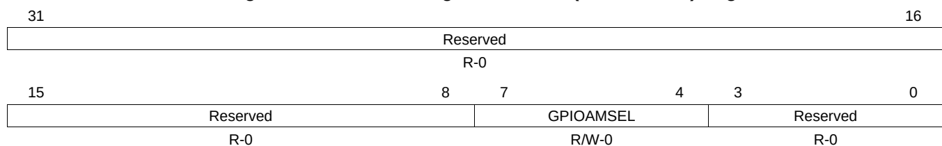
Figure 4-19. GPIO Analog Mode Select (GPIOAMSEL) Register
