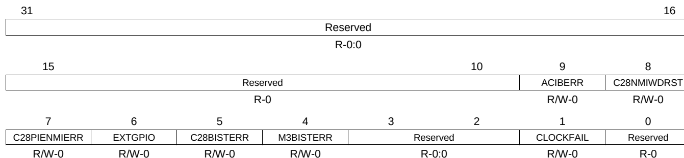
Figure 1-64. M3NMI Flag Force (NMIFLGFRFC) Register
