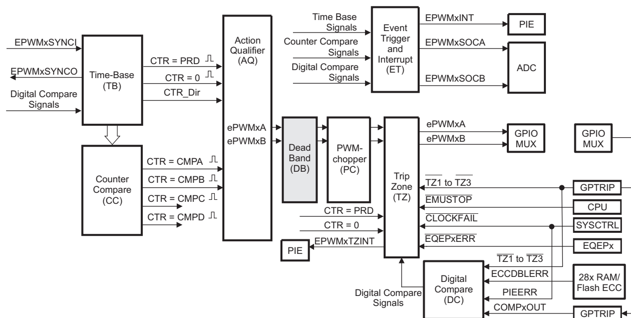
Figure 7-30. Dead_Band Submodule
