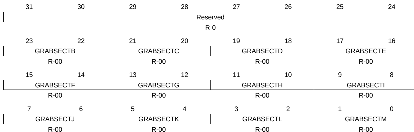
Figure 1-148. Z2_GRABSECTR Register
