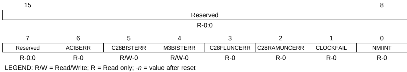
Figure 1-68. C28 NMI Flag (CNMIFLG) Register
