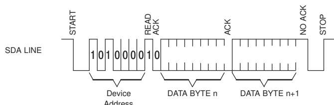
Figure 6-26. Sequential Read
