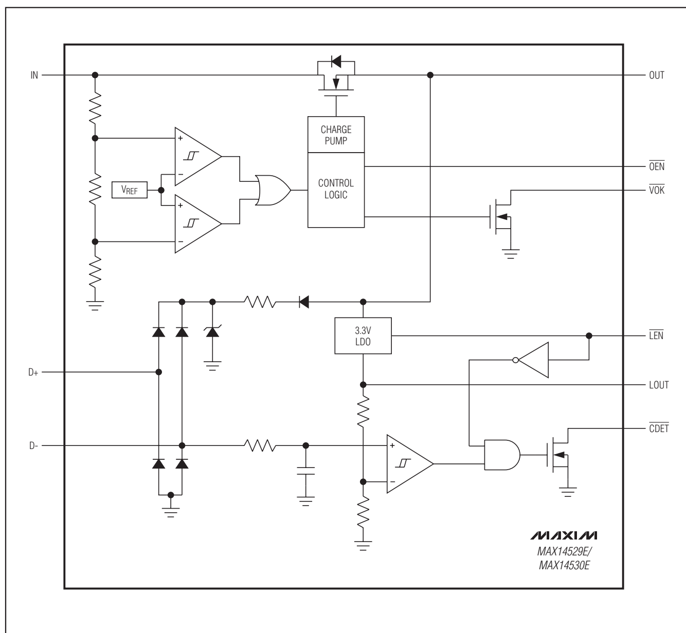
Functional Diagram
