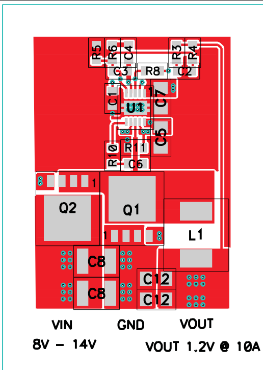
Figure 26. Top Copper With Components
