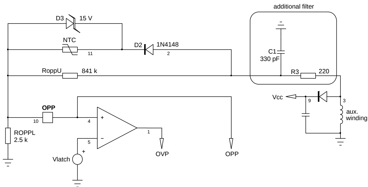
Figure 47. A small RC filter avoids the fast rising spikes from reaching the protection pin of the NCP125x in presence of energetic perturbations superimposed on the input line.
