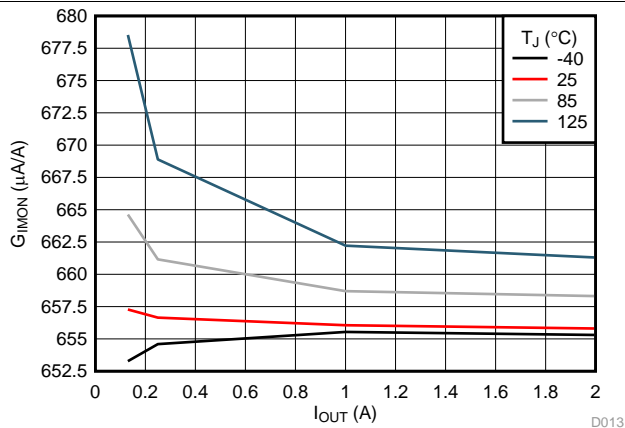
Figure 24. Current Monitor Gain
