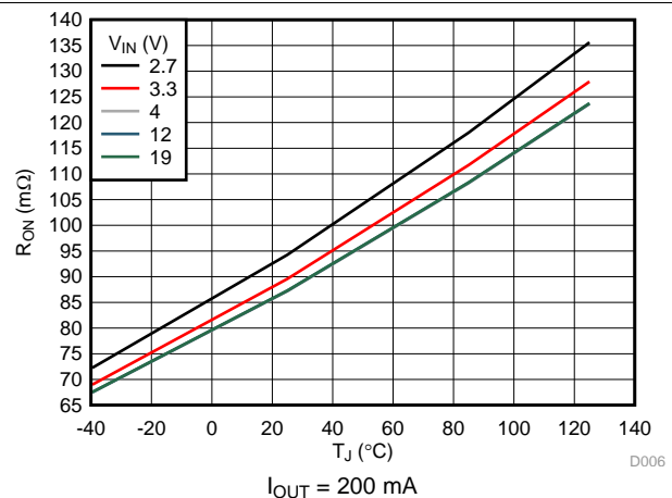
Figure 7. ON Resistance
