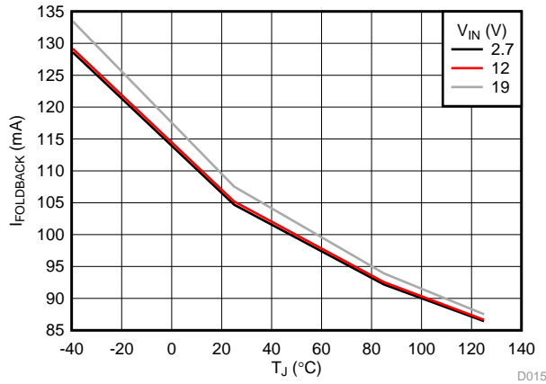
Figure 22. Current Limit Foldback
