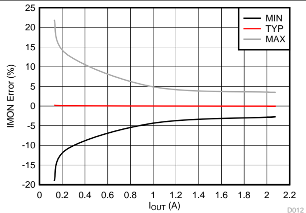
Figure 25. Current Monitor Accuracy
