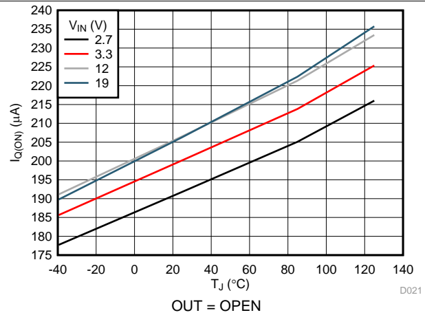
Figure 3. TPS25962x Quiescent Current
