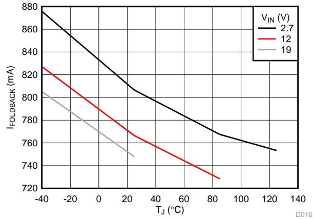
Figure 23. Current Limit Foldback
