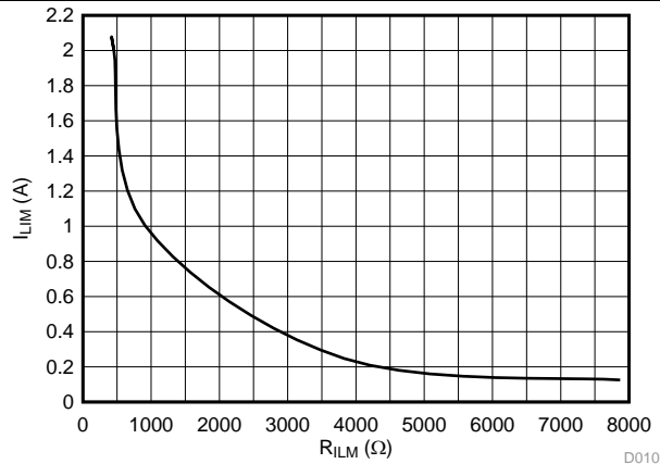
Figure 20. Current Limit vs R_ILM
