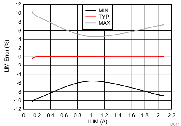
Figure 21. Current Limit Accuracy
