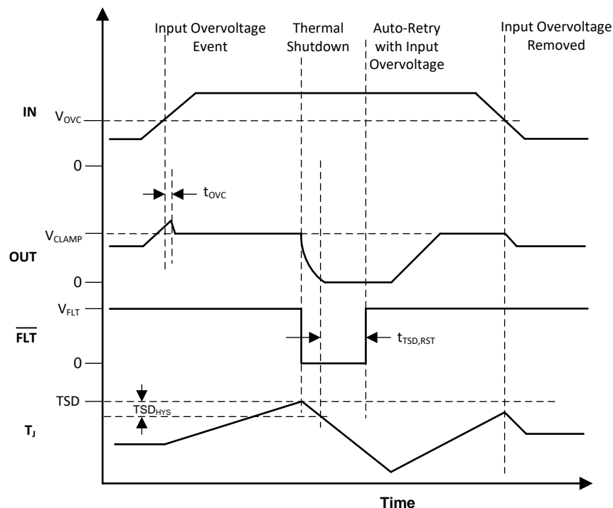
Figure 47. TPS2596x Overvoltage Clamp Response
