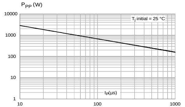
Figure 4: Peak pulse power versus exponential pulse duration (typical values)
