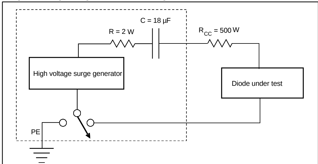
Figure 10: Surge Voltage test circuit according to IEC 61000-4-5 with 500 \Omega serial resistor
