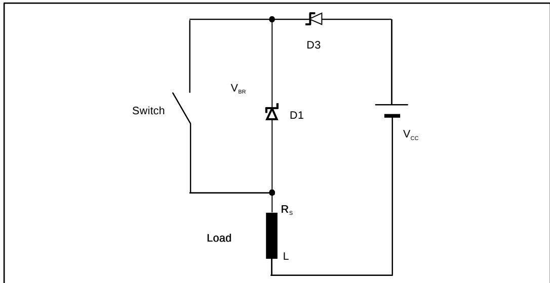
Figure 12: Electrical diagram for inductive load demagnetization
