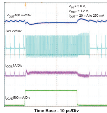
Figure 18. Load Transient PFM Mode 20 mA to 250 mA
