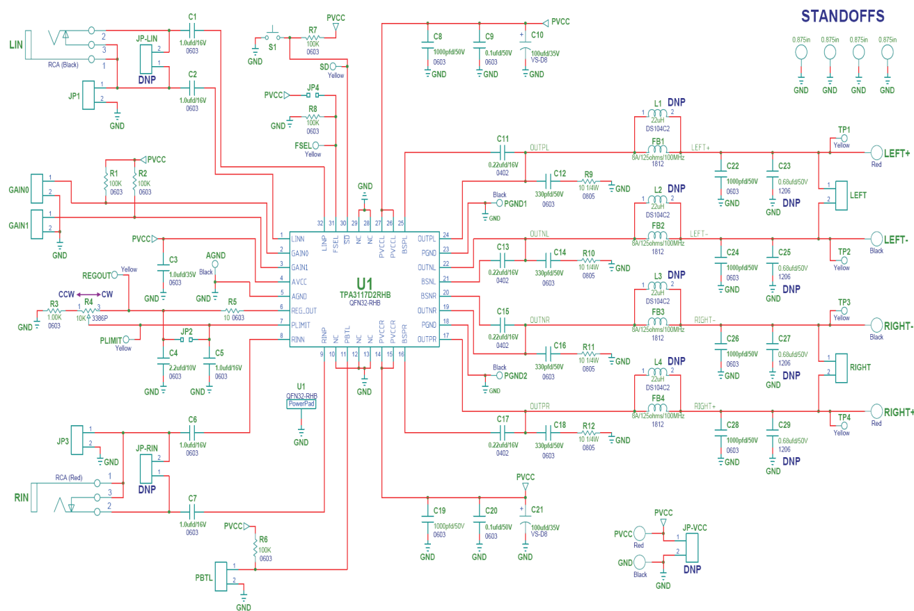
Figure 3. TPA3117D2EVM Schematic
