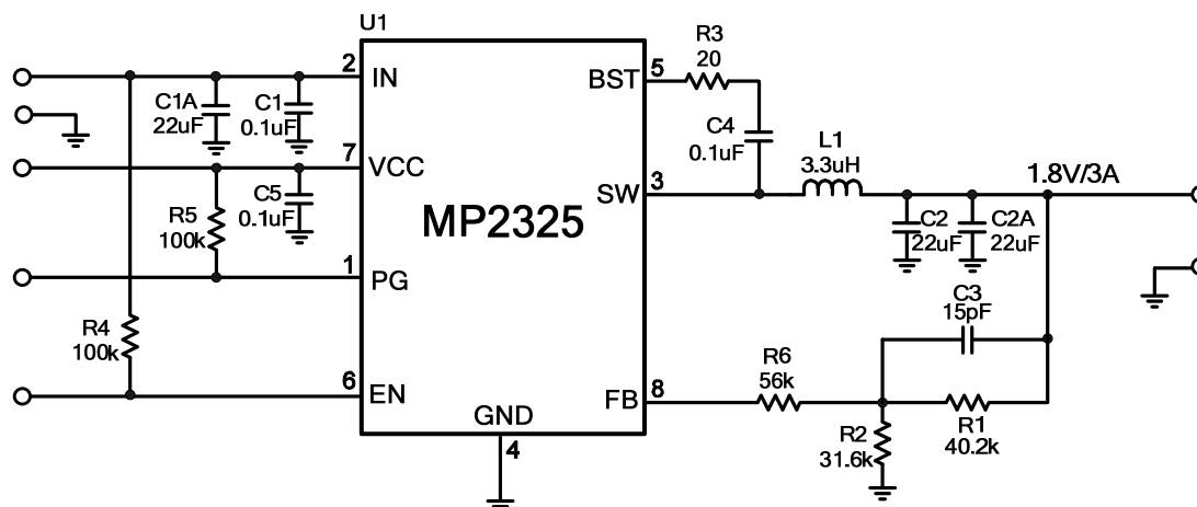
Figure 11: V_o=1.8V , I_o=3A
