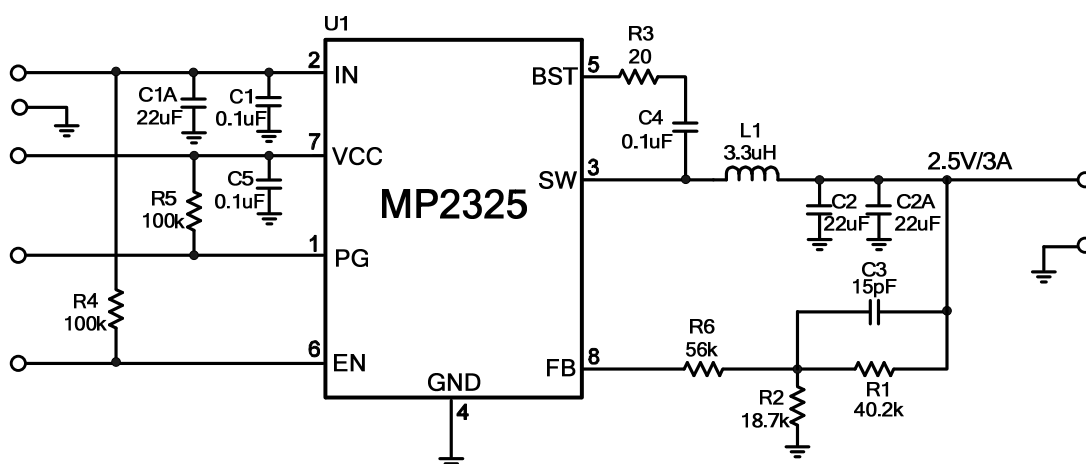
Figure 10: V_o=2.5V , I_o=3A
