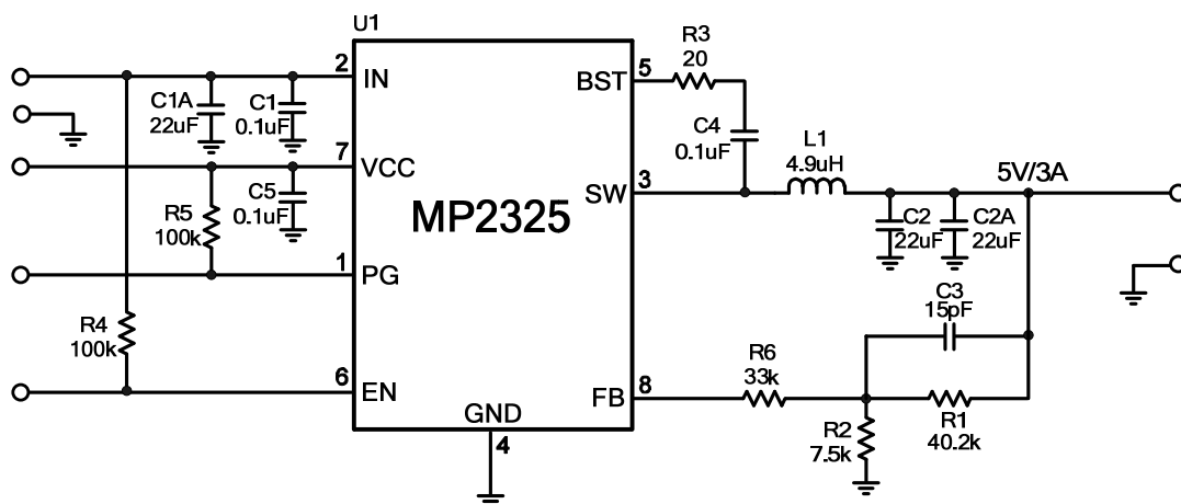
Figure 8: V_o=5V , I_o=3A
