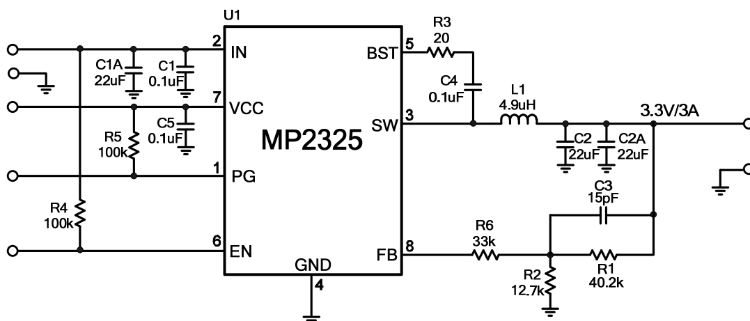
Figure 9: V_o=3.3V , I_o=3A
