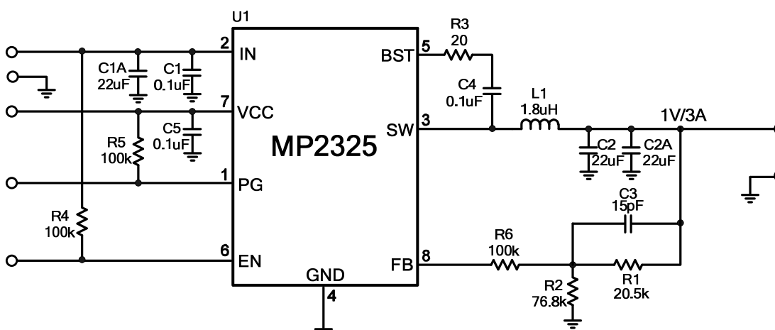
Figure 13: V_o=1V , I_o=3A
