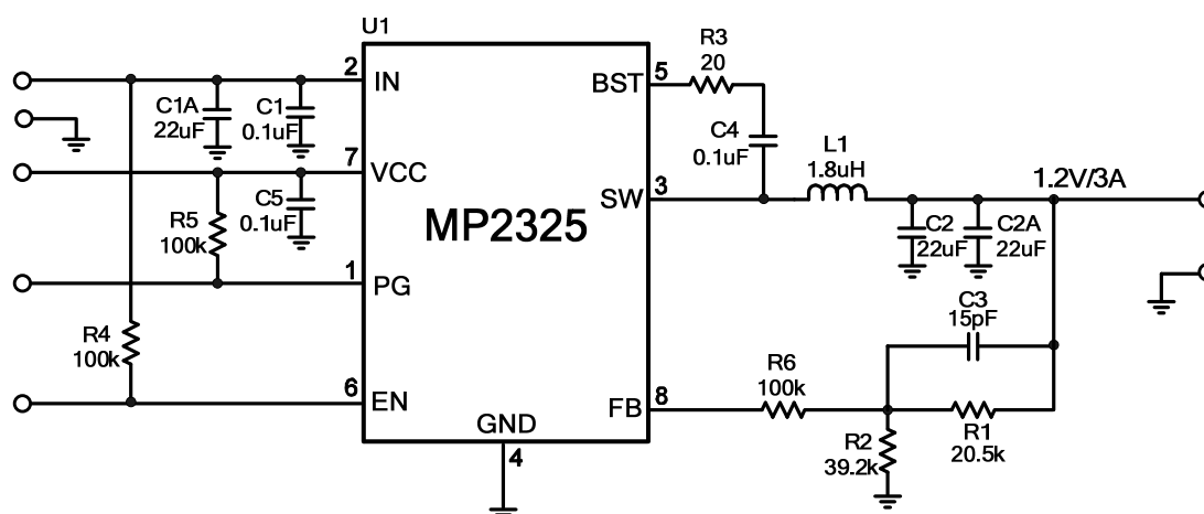
Figure 12: V_o=1.2V , I_o=3A
