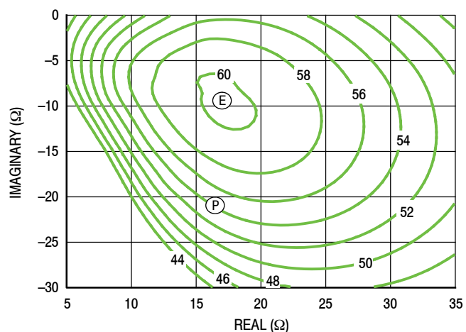
Figure 10. P3dB Load Pull Efficiency Contours (%)
