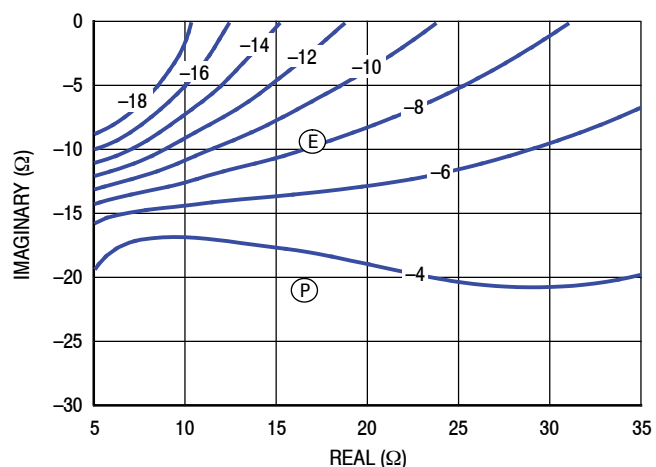
Figure 12. P3dB Load Pull AM/PM Contours (°)
