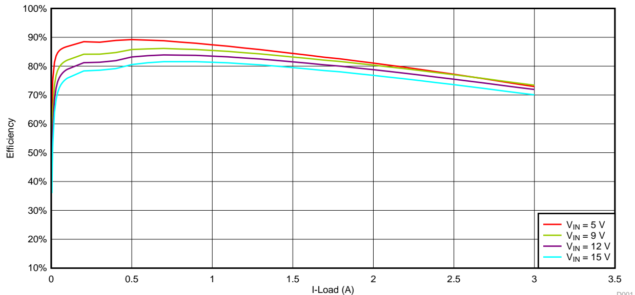
Figure 1. Efficiency
