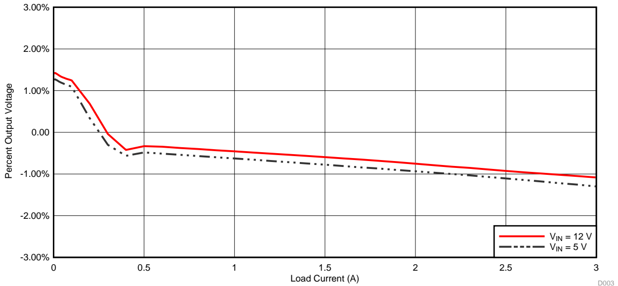
Figure 3. Load Regulation
