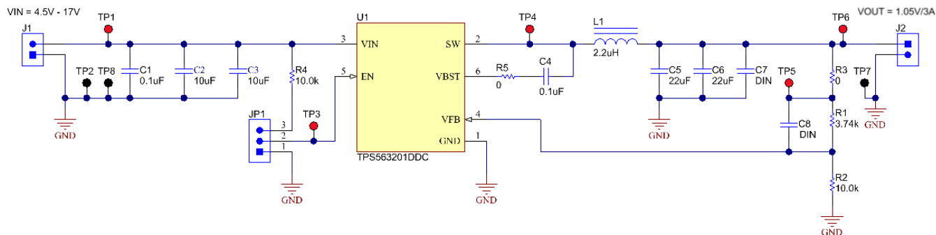
Figure 17. TPS563201EVM-715 Schematic Diagram
