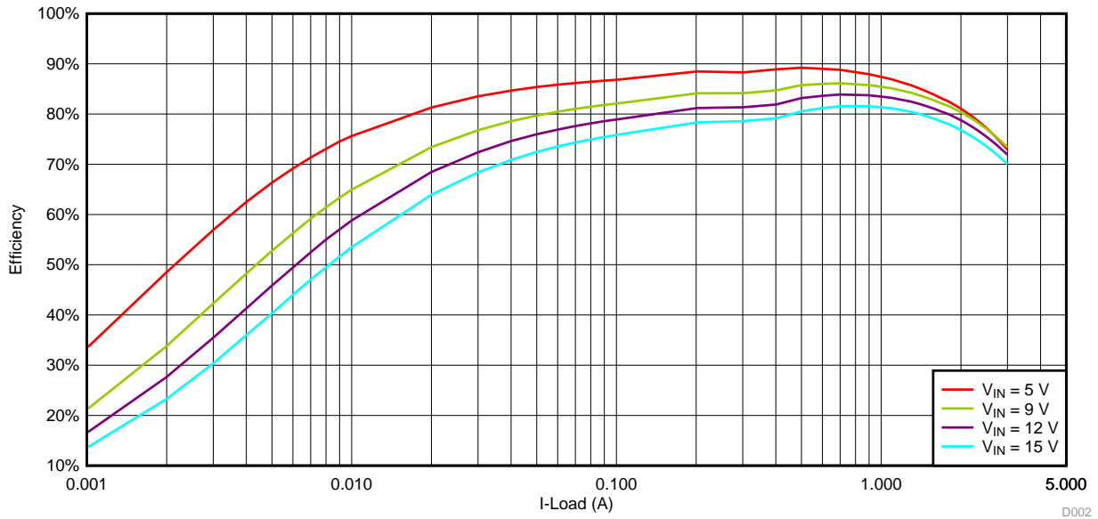
Figure 2. Light Load Efficiency
