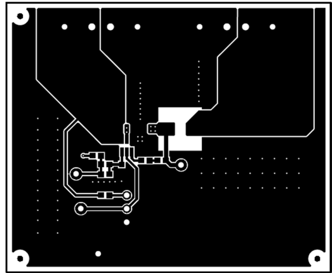
Figure 15. Top Layer
