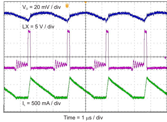
Figure 7. Output Voltage Ripple, I_{OUT} = 250 \text{ mA}
