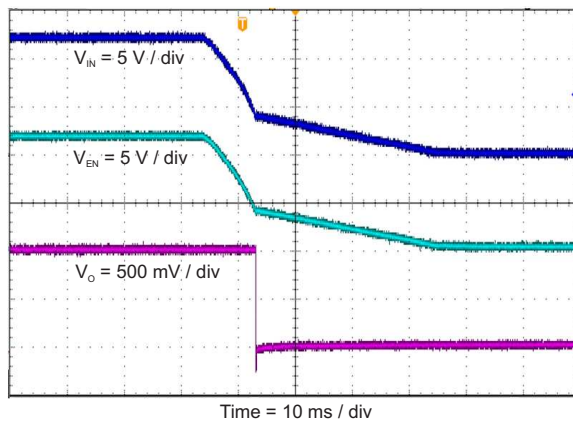
Figure 12. Shut-Down Relative to V_{IN}
