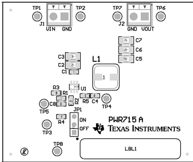
Figure 14. Top Assembly
