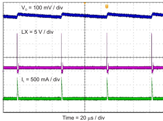
Figure 8. Output Voltage Ripple, I_{OUT} = 10 \text{ mA}
