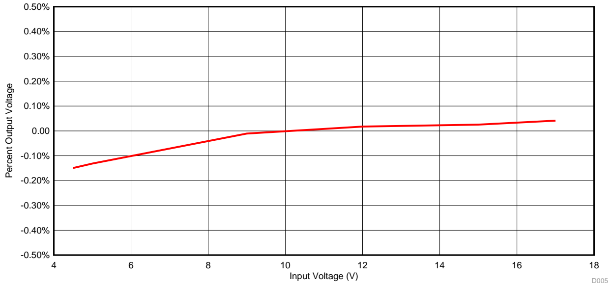
Figure 4. Line Regulation
