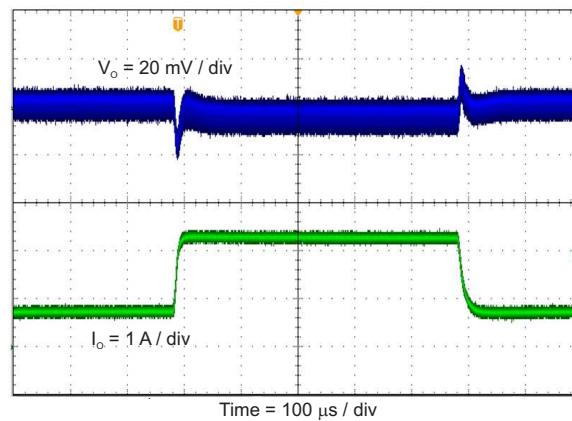
Figure 5. Load Transient Response, 25% to 75% Load Step
