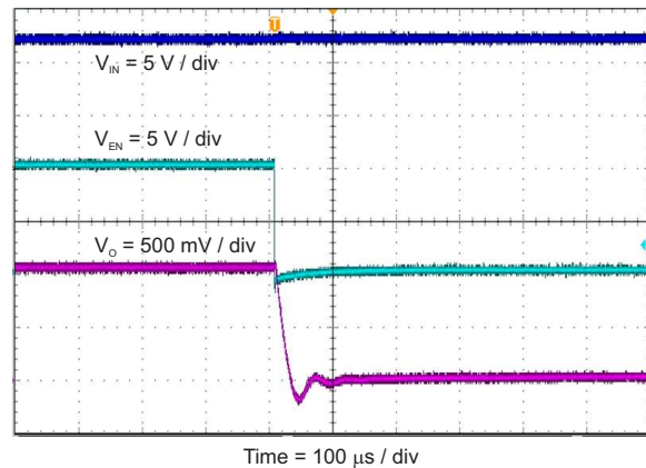
Figure 13. Shut-Down Relative to EN
