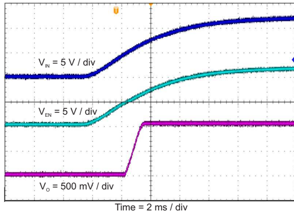
Figure 10. Start-Up Relative to V_{IN}
