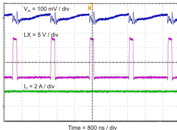
Figure 9. Input Voltage Ripple, I_{OUT} = 3 \text{ A}
