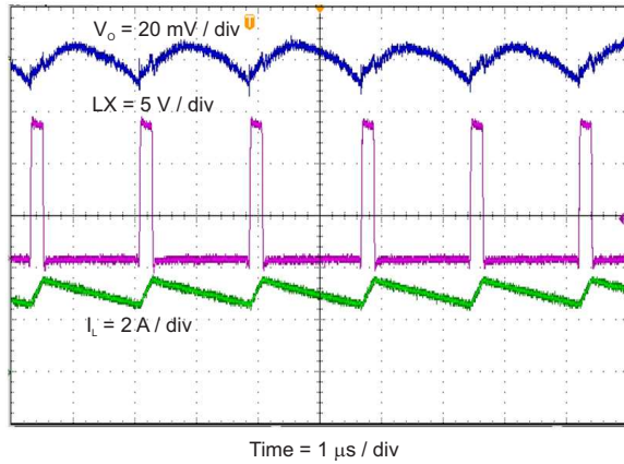
Figure 6. Output Voltage Ripple, I_{OUT} = 3 \text{ A}
