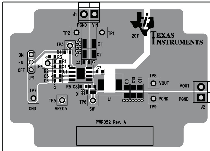
Figure 13. Top Assembly
