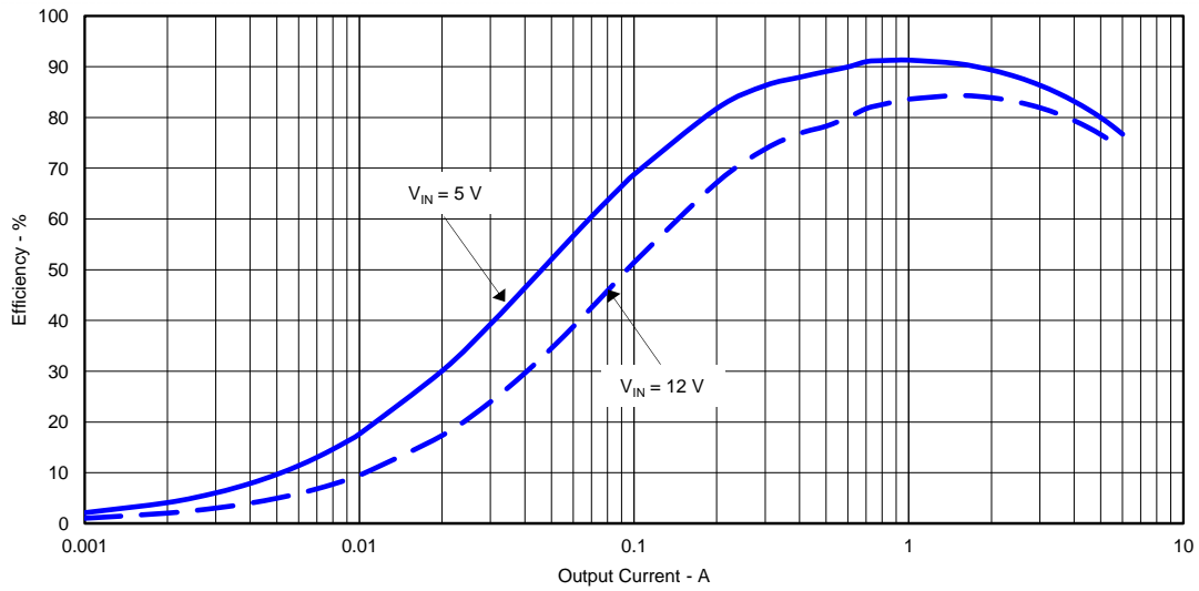
Figure 2. TPS54627EVM-052 Light-Load Efficiency
