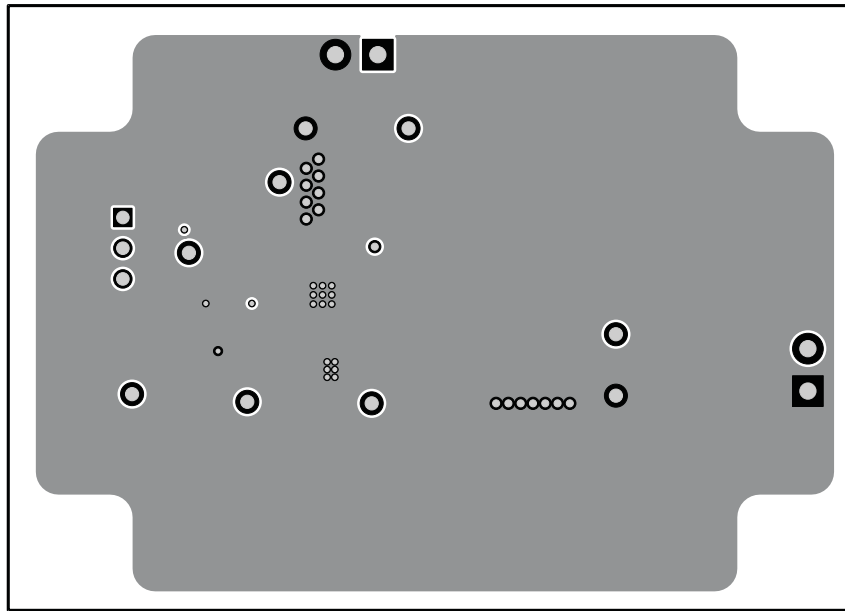
Figure 16. Internal Layer 2
