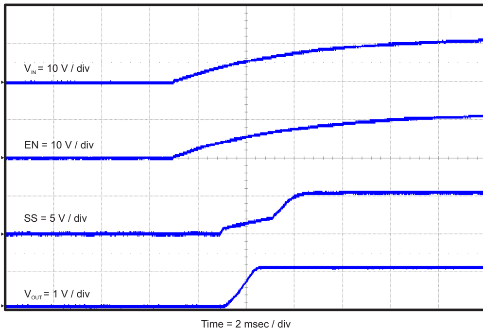
Figure 9. TPS54627EVM-052 Start-Up Relative to V_{IN} with SS
