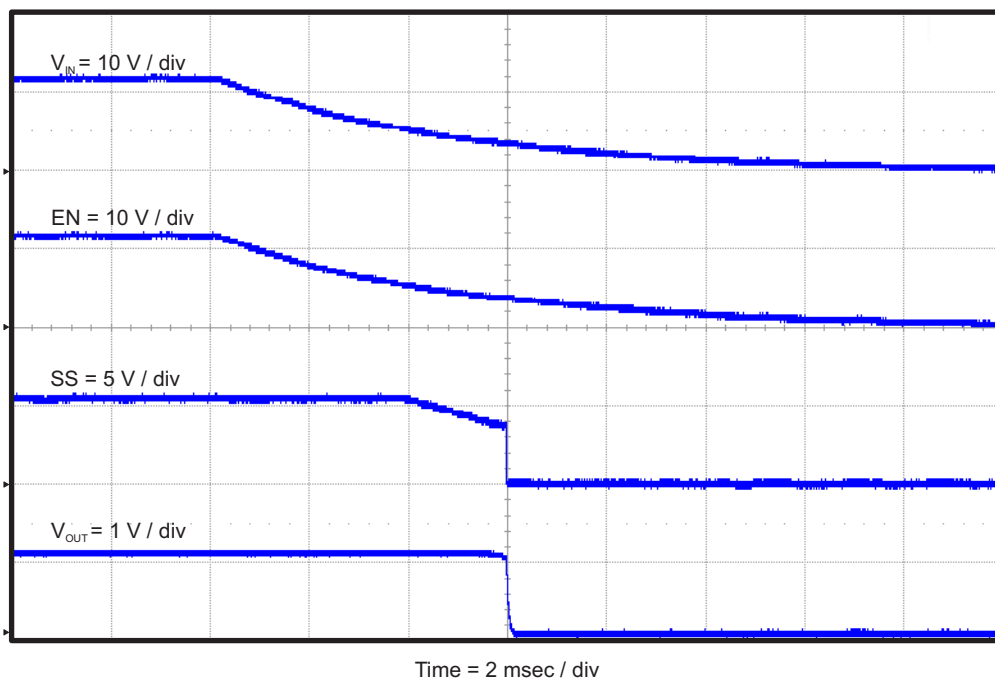
Figure 11. TPS54627EVM-052 Shut-Down Relative to V_{IN} with SS
