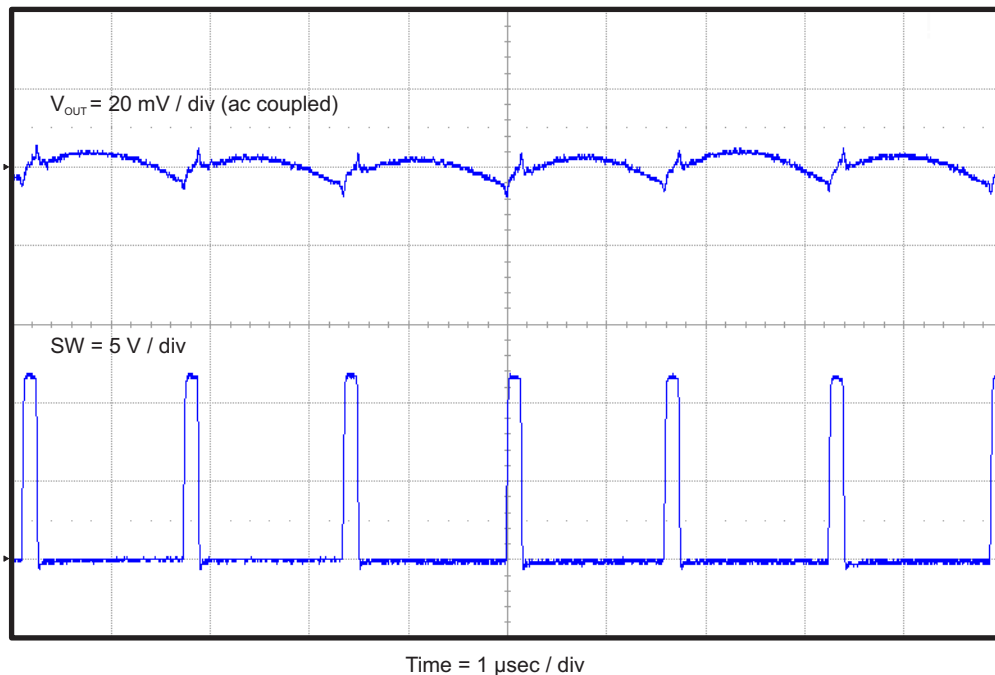
Figure 7. TPS54627EVM-052 Output Voltage Ripple ( I_{OUT} = 100 \text{ mA} )
