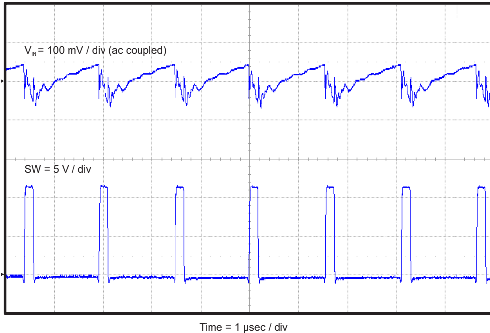
Figure 8. TPS54627EVM-052 Input Voltage Ripple
