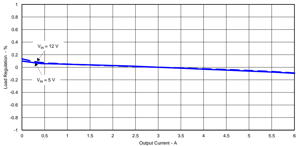
Figure 3. TPS54627EVM-052 Load Regulation, V_{IN} = 5\text{ V} and V_{IN} = 12\text{ V}
