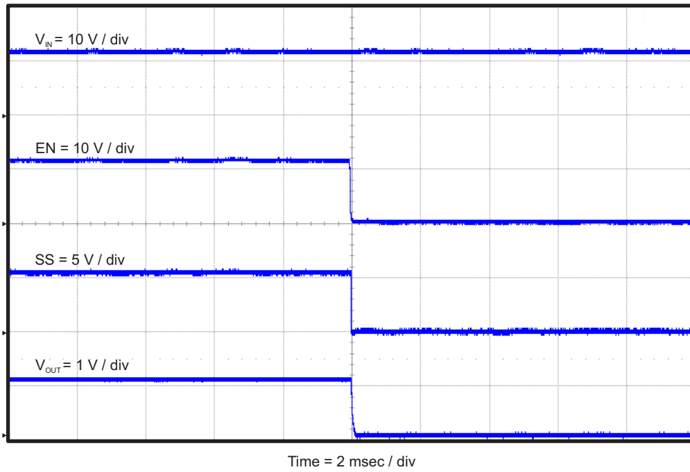
Figure 12. TPS54627EVM-052 Shut-Down Relative to EN with SS
