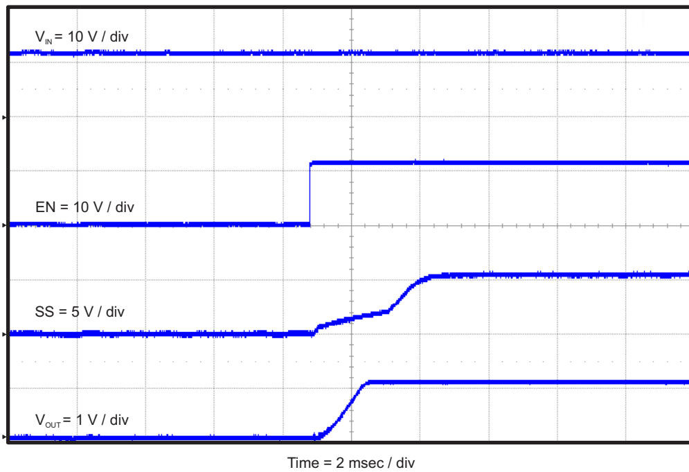
Figure 10. TPS54627EVM-052 Start-Up Relative to EN with SS
