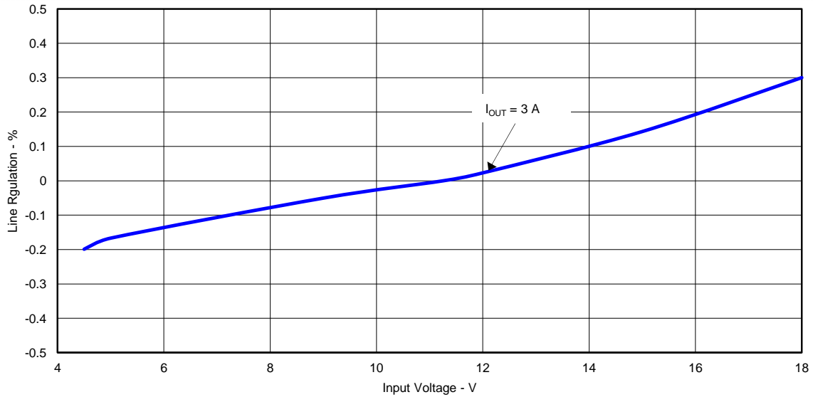
Figure 4. TPS54627EVM-052 Line Regulation
