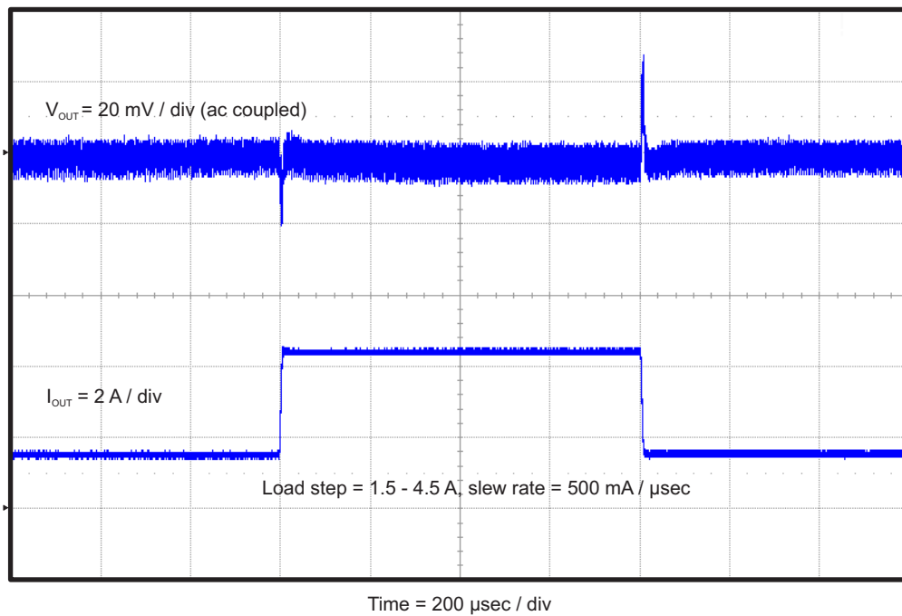
Figure 5. TPS54627EVM-052 Load Transient Response
