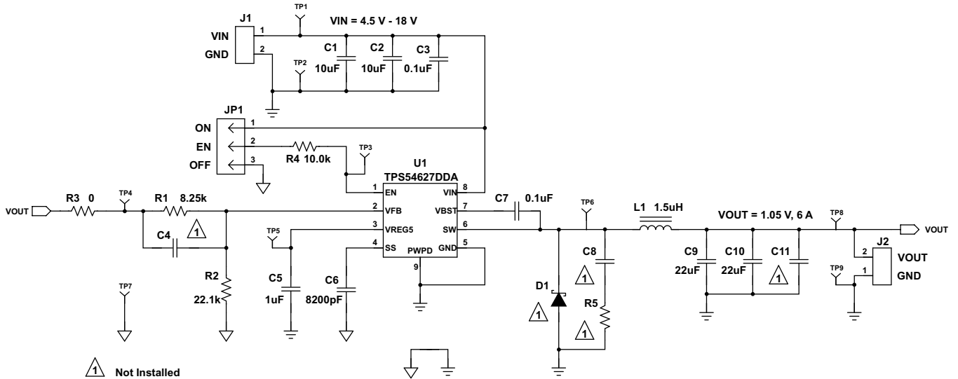
Figure 18. TPS54627EVM-052 Schematic Diagram
