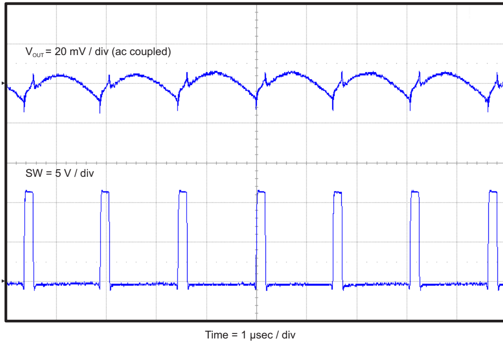
Figure 6. TPS54627EVM-052 Output Voltage Ripple ( I_{OUT} = 2 \text{ A} )
