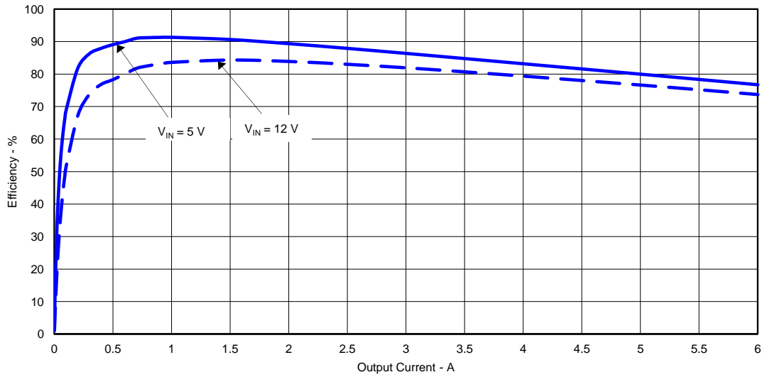
Figure 1. TPS54627EVM-052 Efficiency
