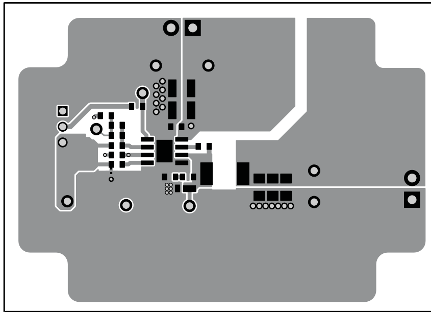
Figure 14. Top Layer
