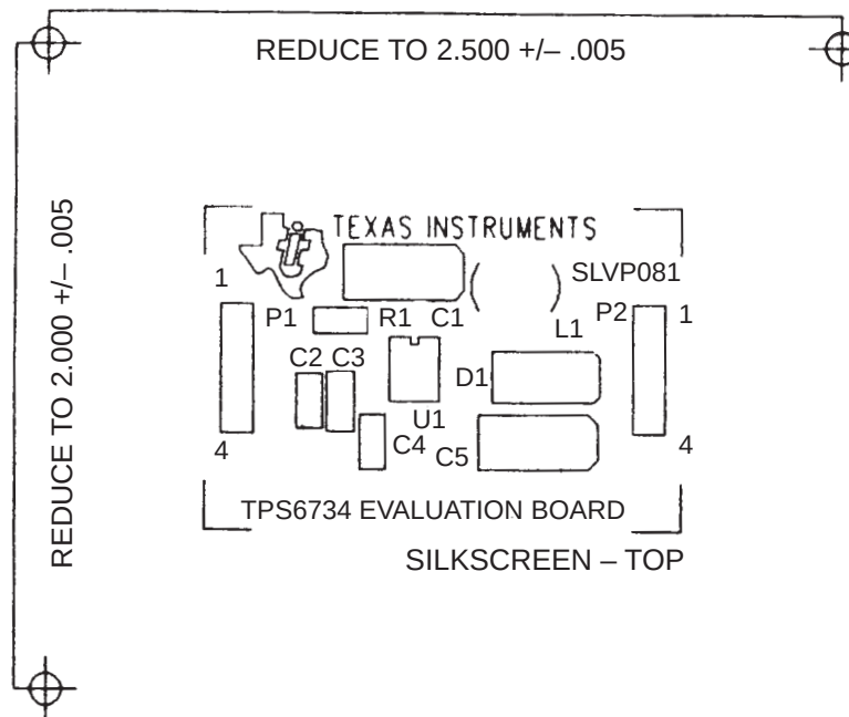
Figure 14. Component Placement
