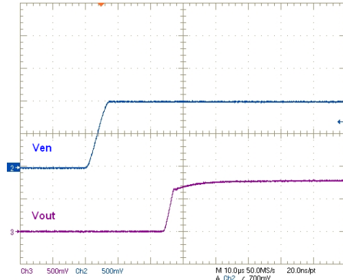
Figure 15. Enable transient
