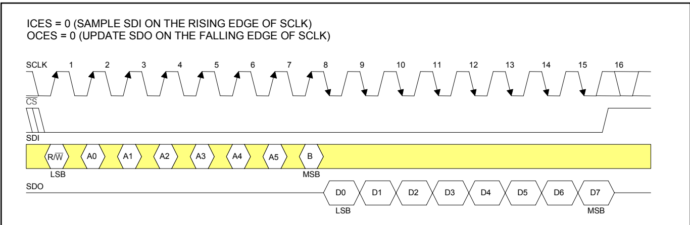
Figure 6-4. Serial Port Operation Mode 4
