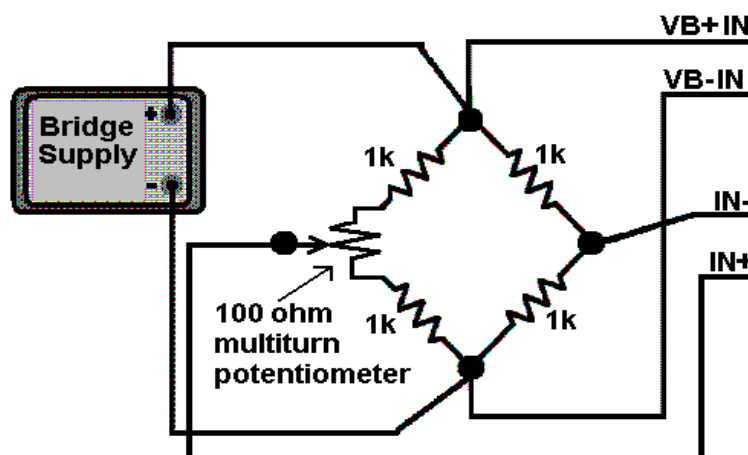
Figure 4. A Wheatstone Bridge
