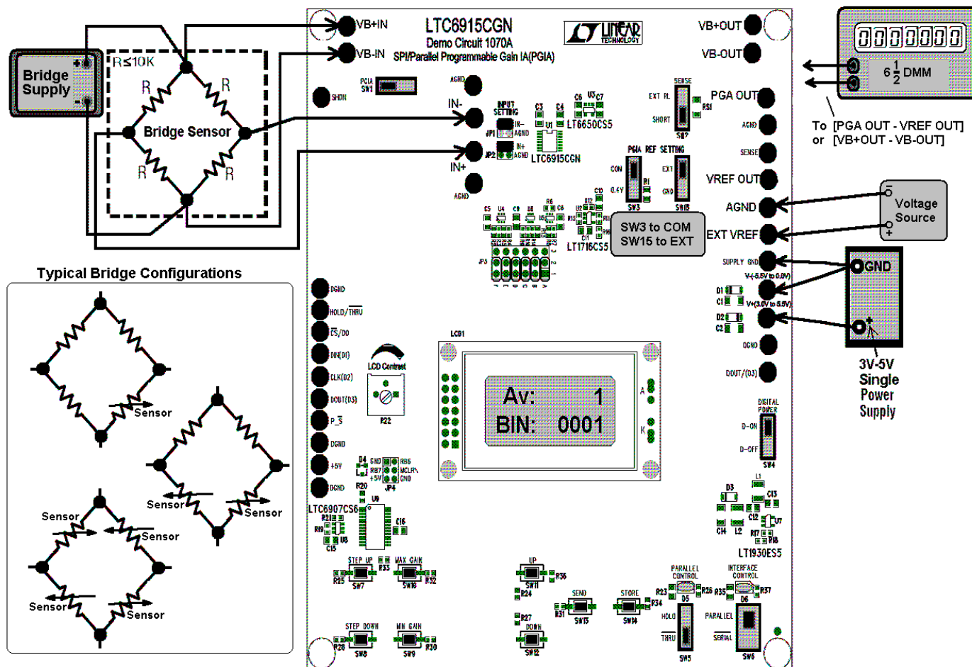
Figure 3. Test Setup Using a Bridge Sensor
