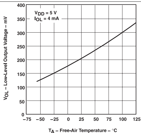
Figure 8. Low-Level Output Voltage vs Free-Air Temperature
