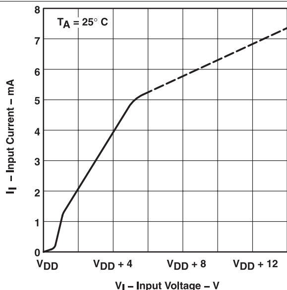
Figure 22. Input Current vs Input Voltage
