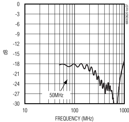
MAX3620C S11
