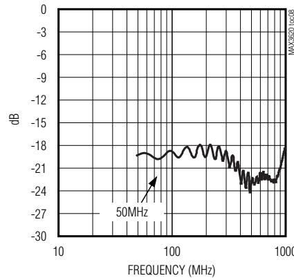
MAX3620D S11
