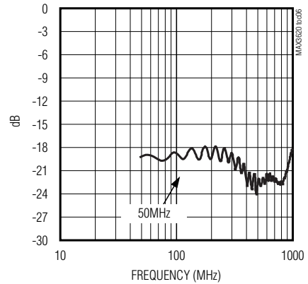
MAX3620B S11
