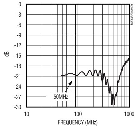
MAX3620A S22
