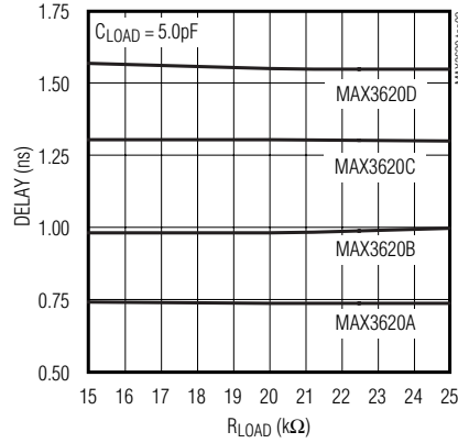
DELAY vs. R_{LOAD} (HIGH LOAD RESISTANCE)
