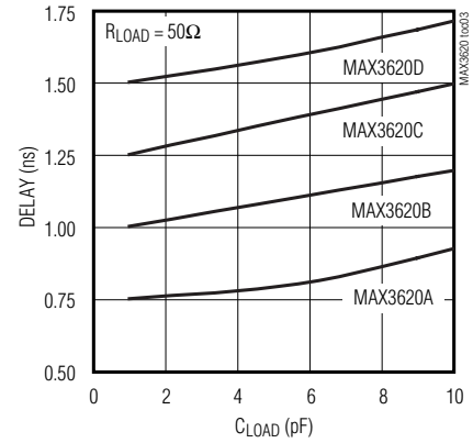
DELAY vs. C_{LOAD} (LOW LOAD RESISTANCE)
