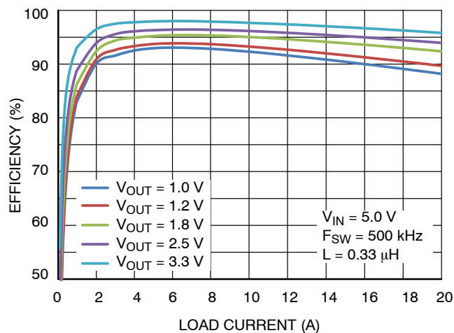
Figure 7. Efficiency vs. Load Current ( V_{IN} = 5.0\text{ V} ), Inductor: Würth Electronics 7443320033
