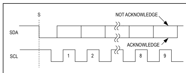
Figure 6. Acknowledge Bits
