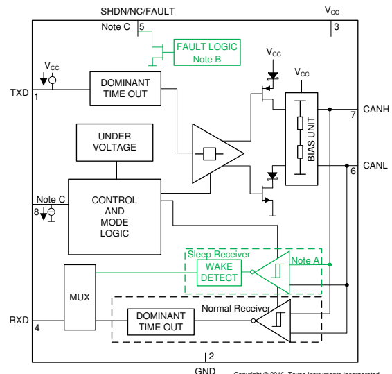
Block Diagram
