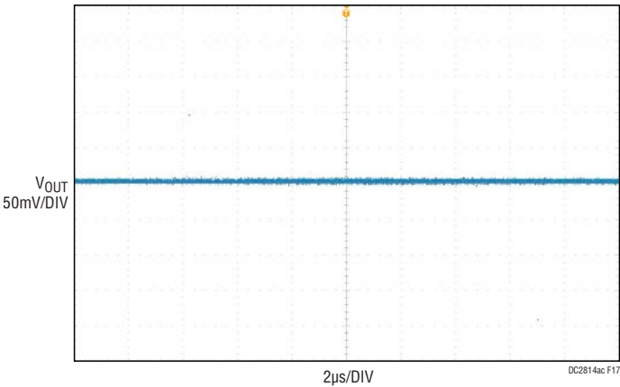
Figure 17. DC2814A-C Output Voltage Ripple at 45V IN (Pass-Thru), 45V OUT , 2A Load Current
