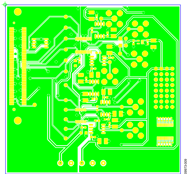
Figure 9. Component-Side Artwork
