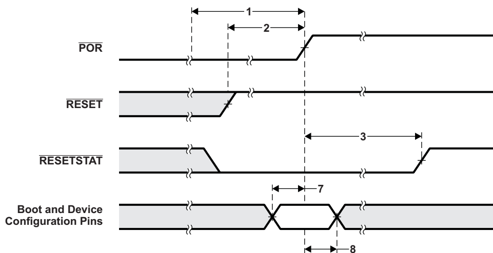
Figure 7-10 Warm Reset Timing — RESETSTAT Relative to RESET
