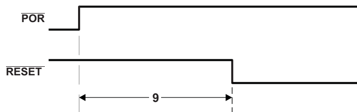
Figure 7-11 Warm Reset Timing — Setup Time Between POR De-Asserted and RESET Asserted
