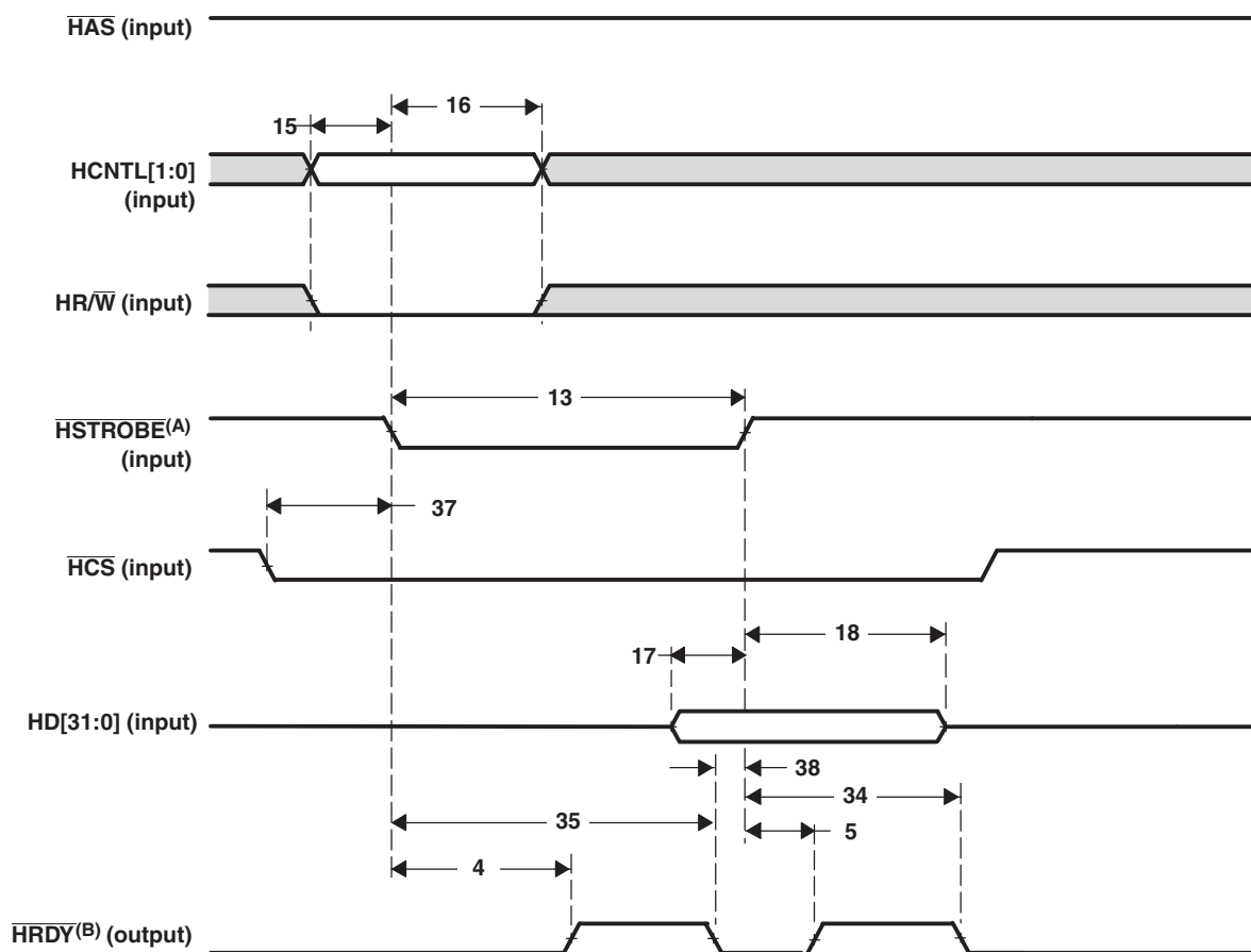
Figure 7-34 HPI32 Write Timing (HAS Not Used, Tied High)
