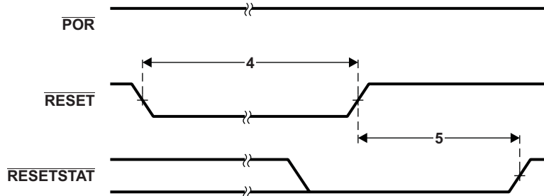
Figure 7-11 Warm Reset Timing — Setup Time Between POR De-Asserted and RESET Asserted
