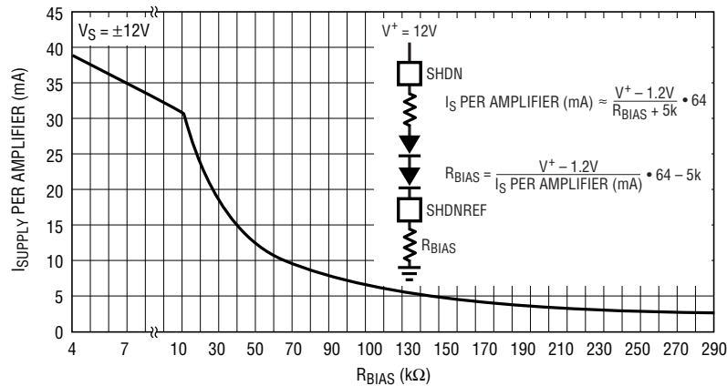
Figure 3. R_{\text{BIAS}} to Ground Current Control
