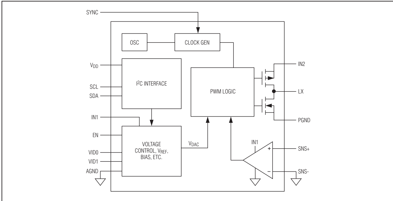
Figure 1. Block Diagram
