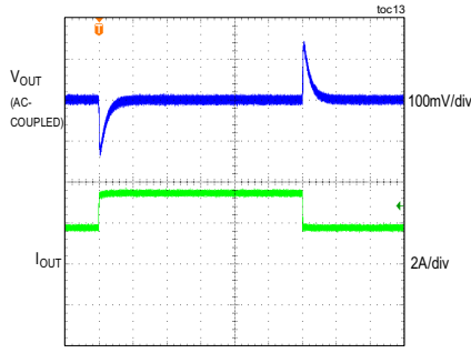
LOAD TRANSIENT BETWEEN 1.75A AND 3.5A
