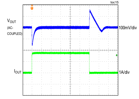
LOAD TRANSIENT BETWEEN 0A AND 1.75A
