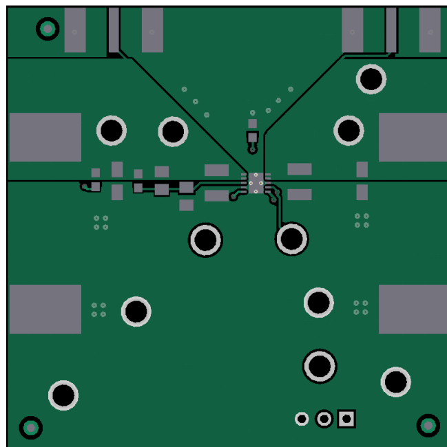
Figure 4. Top-Layer Routing
