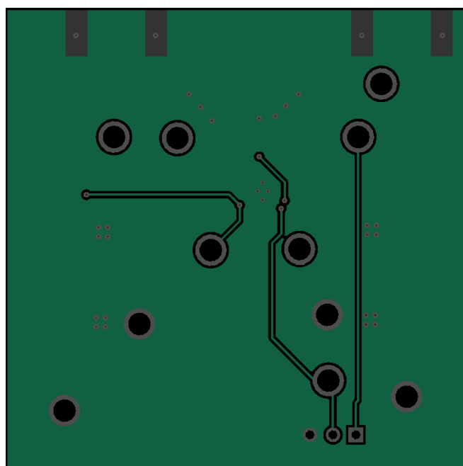
Figure 7. Bottom-Layer Routing
