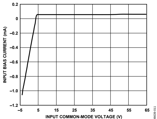
Figure 10. Input Bias Current vs. Input Common-Mode Voltage Per Input
