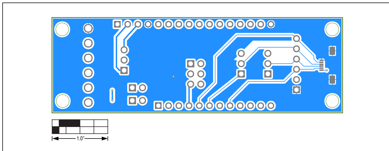
MAX31889 EV Kit Interface Board PCB Layout—Bottom View
