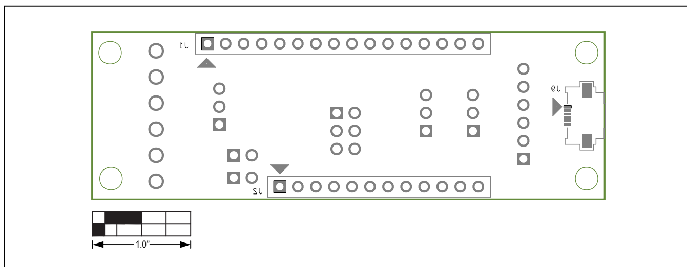
MAX31889 EV Kit Interface Board PCB Layout—Bottom Silkscreen
