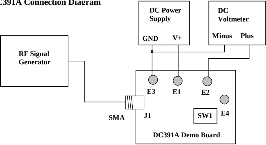
DC391A Connection Diagram
