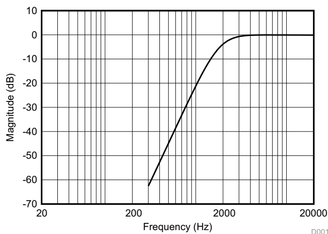
Figure 13. High-Pass Filter Frequency Response
