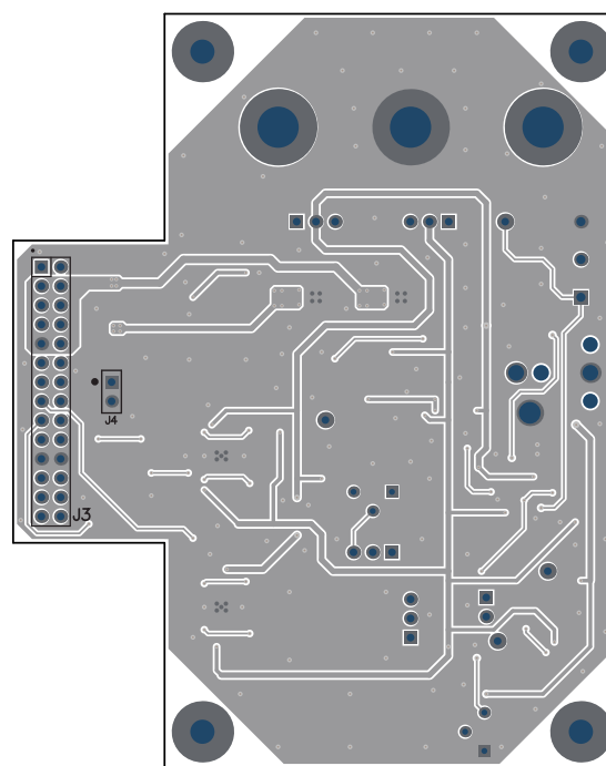
Figure 20. Bottom Overlay
