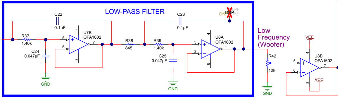
Figure 7. Low-Pass Filter Schematic
