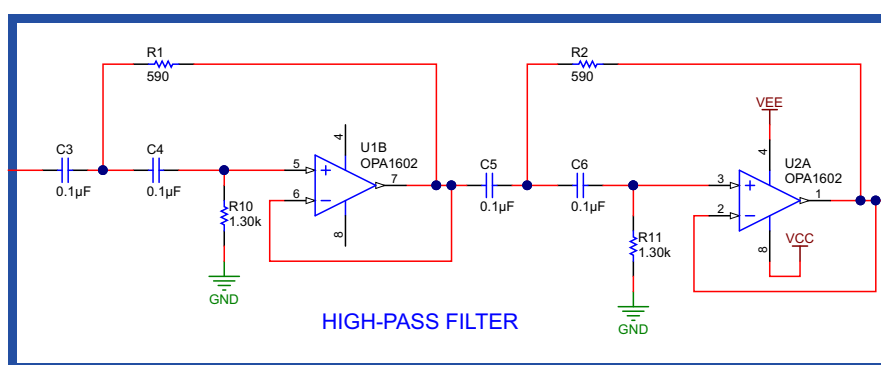
Figure 12. High-Pass Filter Schematic
