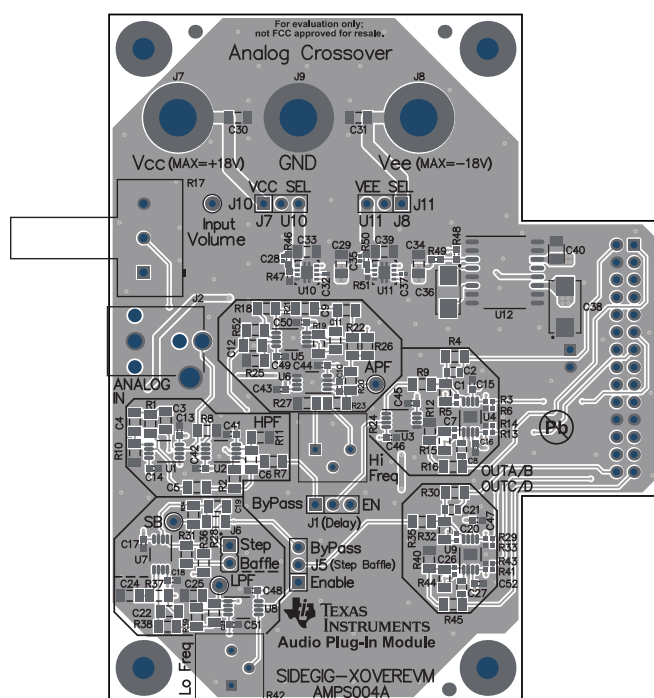
Figure 19. Top Overlay
