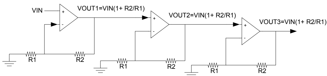
Figure 23.8. Cascaded Non-inverting PGA Overview
