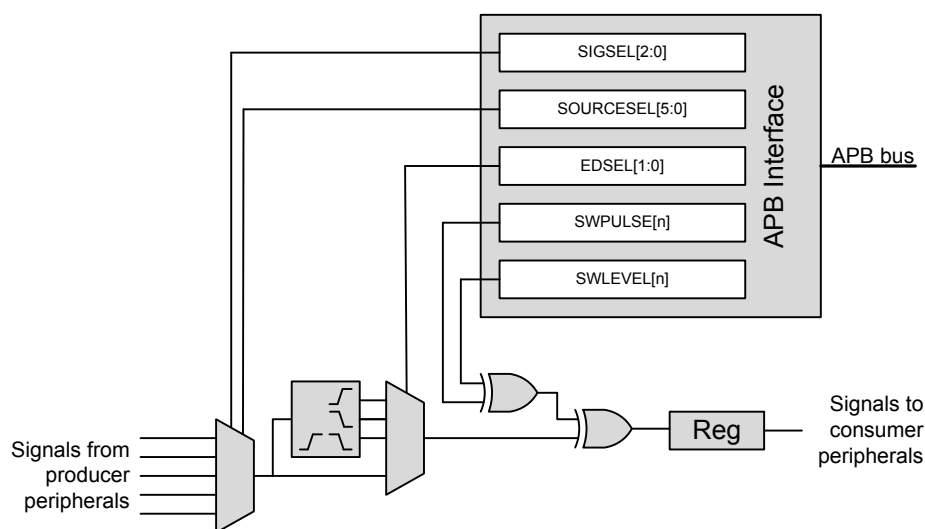
Figure 14.1. PRS Overview
