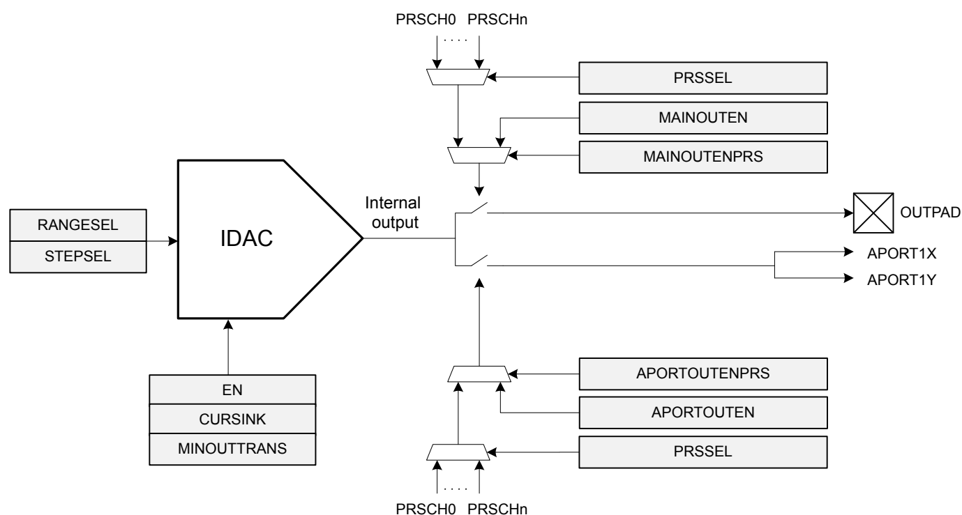
Figure 26.1. IDAC Overview
