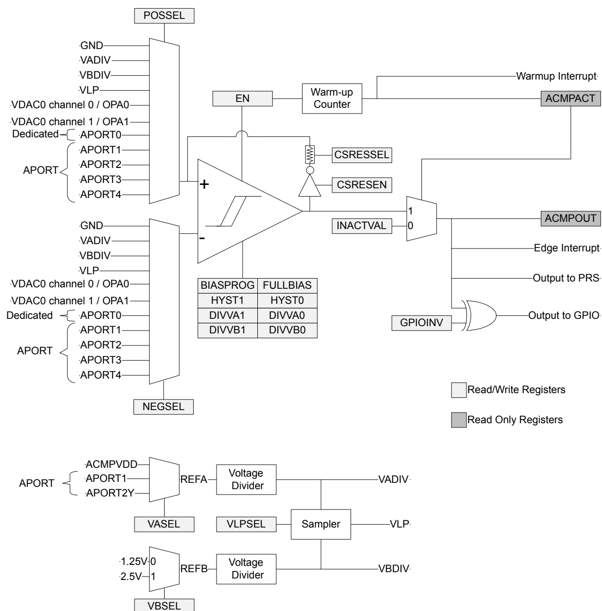
Figure 24.1. ACMP Overview
