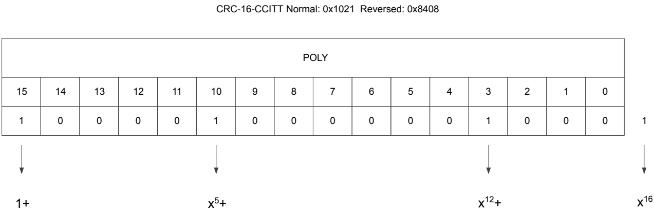
Figure 28.2. Polynomial Representation
