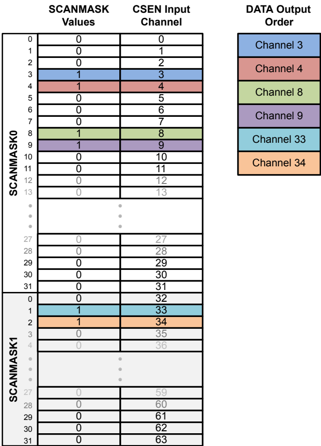
Figure 33.4. Scan Mode Sequencing
