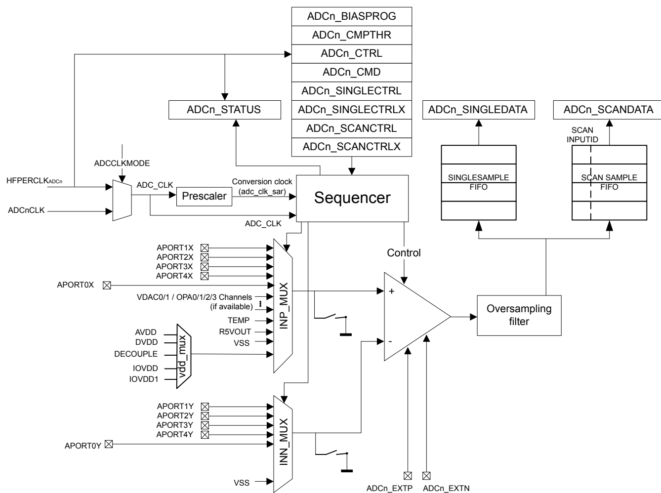
Figure 25.1. ADC Overview
