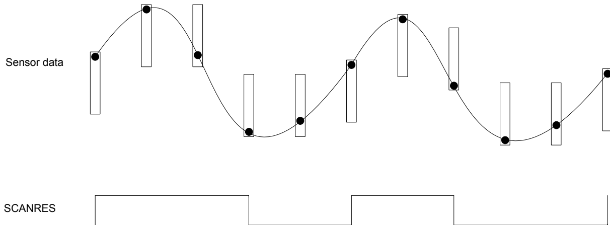
Figure 27.8. Sliding Window
