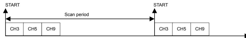
Figure 27.3. Scan Sequence
