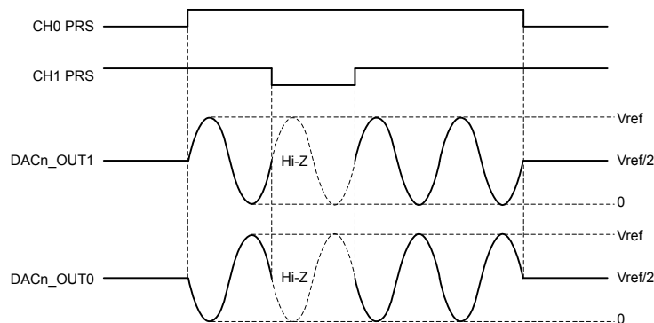
Figure 22.6. VDAC Sine Mode
