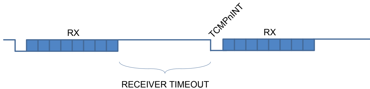
Figure 17.27. USART RX Timeout
