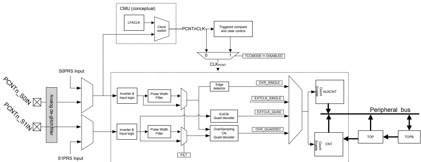
Figure 15.1. PCNT Overview
