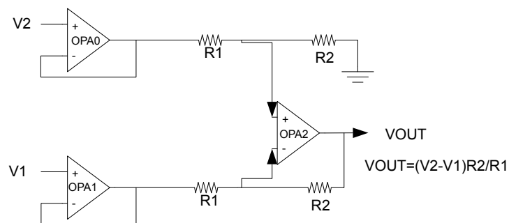
Figure 23.10. Three Op-amp Differential Amplifier Overview
