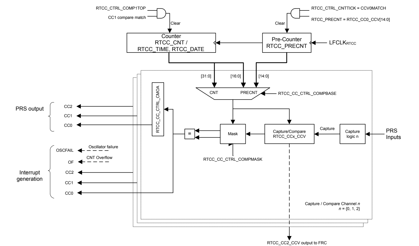
Figure 12.1. RTCC Overview
