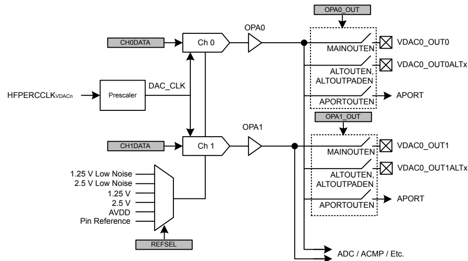
Figure 22.1. VDAC Overview
