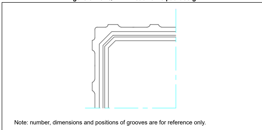
Figure 52. eTQFP144 leadframe pad design
