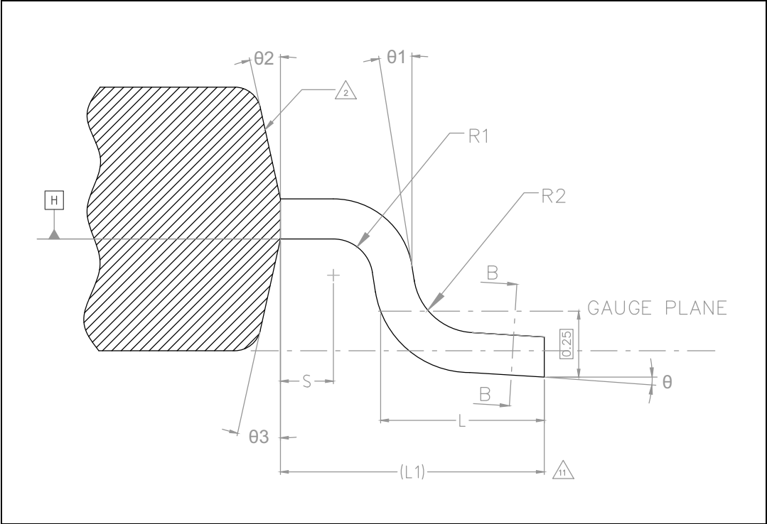
Figure 46. eLQFP176 section A-A
