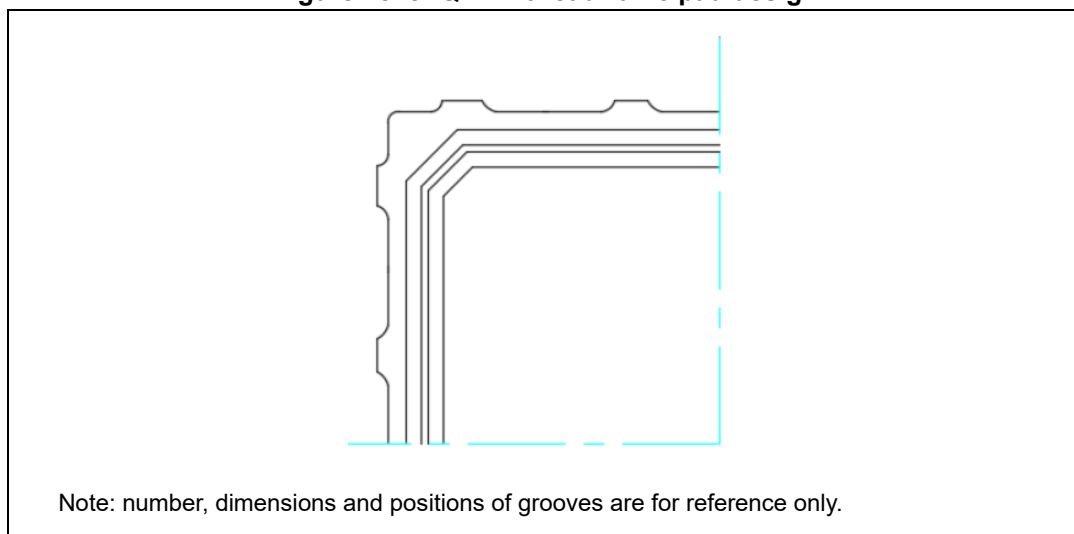
Figure 48. eLQFP176 leadframe pad design
