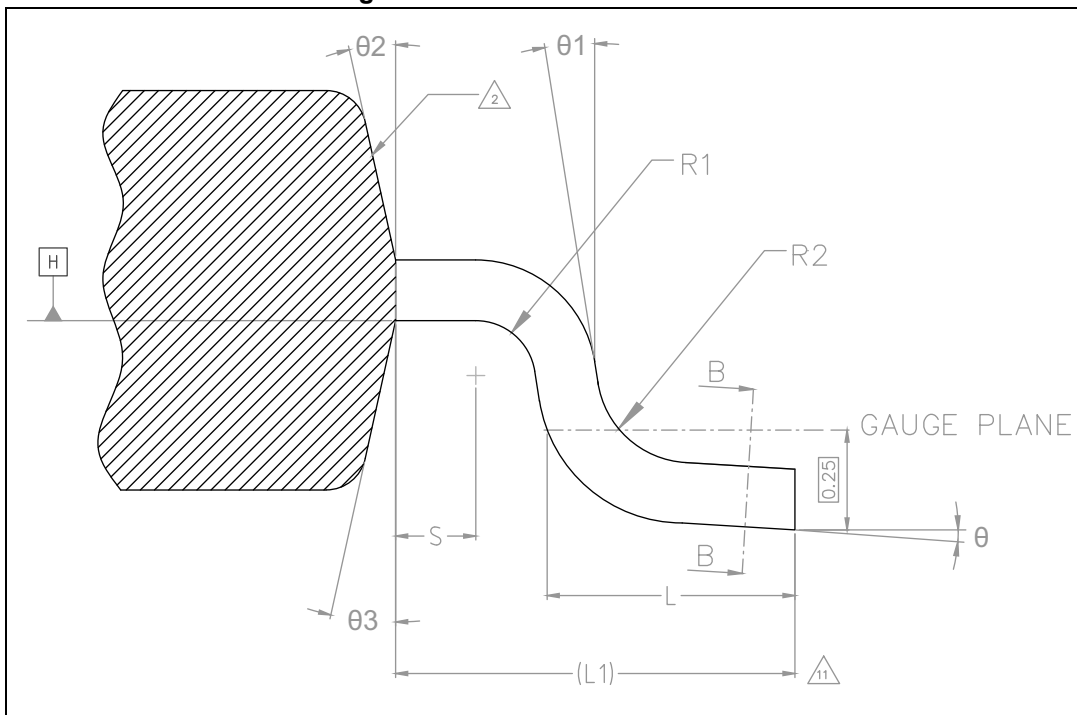
Figure 50. eTQFP144 section A-A
