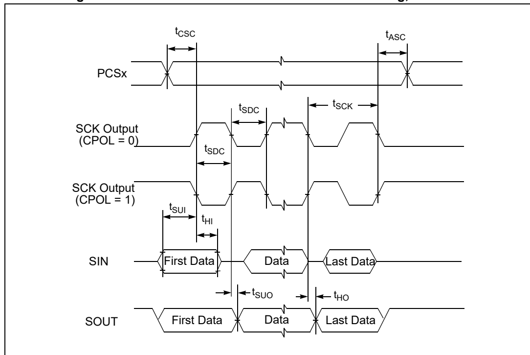
Figure 28. DSPI CMOS master mode — modified timing, CPHA = 0
