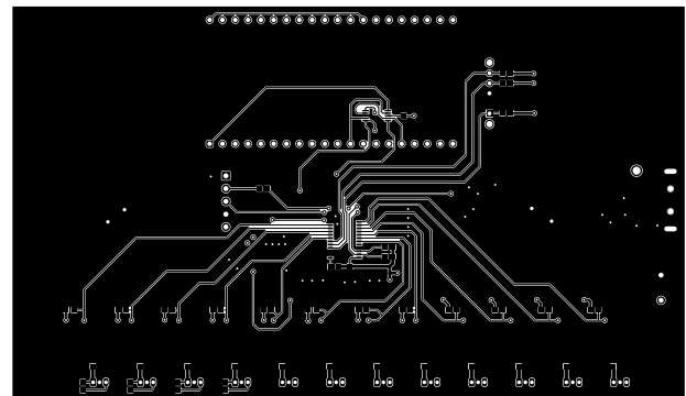
Figure 10. Bottom Layer
