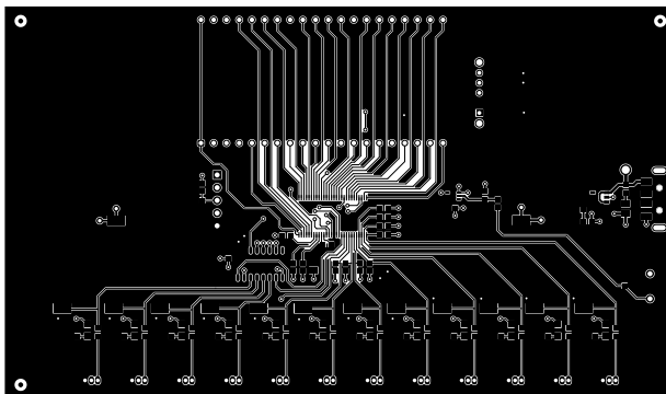
Figure 8. Top Layer
