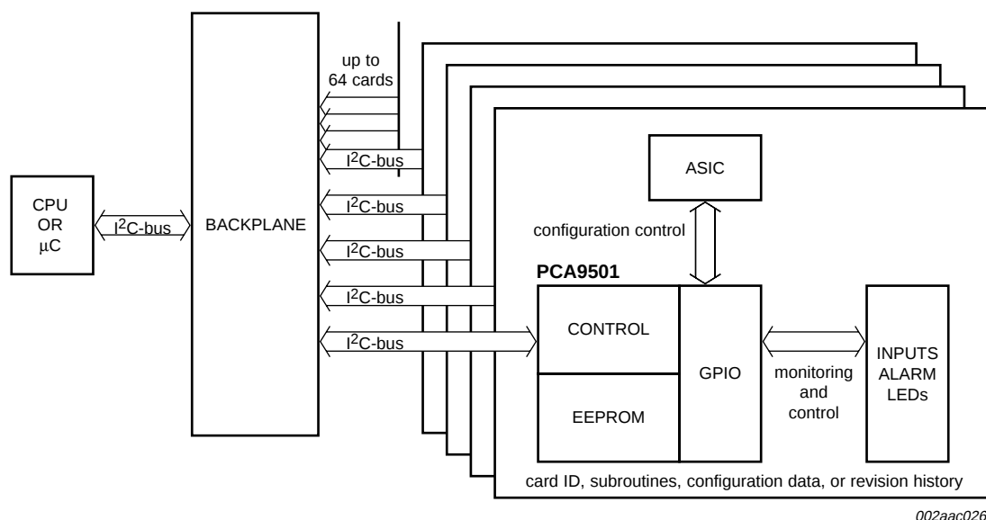
Fig 21. PCA9501 used as interface for board configuration
