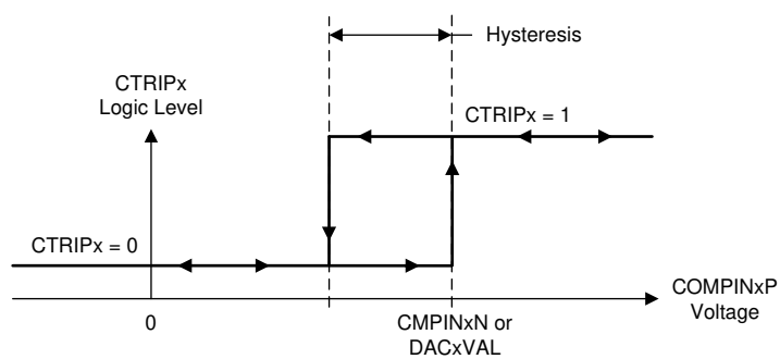
Figure 5-36. CMPSS Comparator Hysteresis
