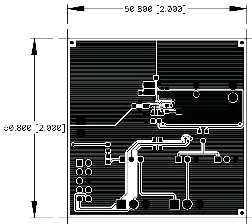
Figure 5. Top Layer
